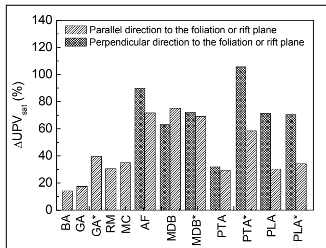
Figure 4. Increase of the UPV in saturated specimens with respect to the dry specimens
