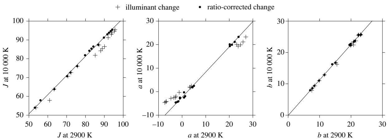
Figure 4. Values of appearance attributes of lightness J , redness-greenness a , and yellowness-blueness b in the approximately uniform colour space CAM02-UCS [43] corresponding to the L, M, and S cone excitations in figure 2. The fitted line is a locally weighted linear regression [49,50]. Other details as for figure 2.
