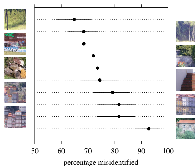
Figure 6. Percentage of misidentifications of illuminant changes for each scene. Symbols show percentages averaged over observers and relative deviations in spatial cone-excitation ratios from 2.5% to 6.5%. Error bars mark 95% confidence intervals [53]. The guessing misidentification rate was 50%.
