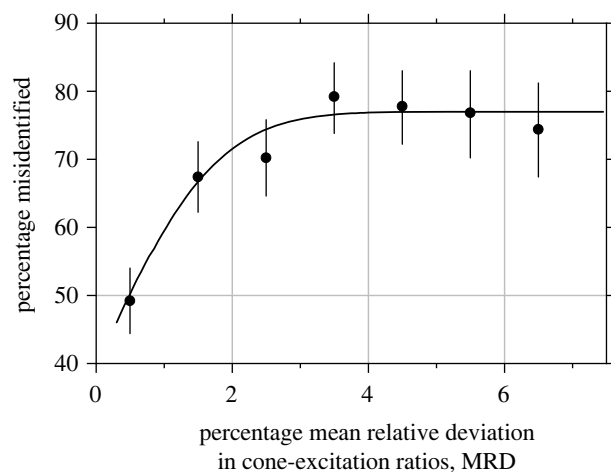
Figure 5. Percentage of misidentifications of illuminant changes on scenes as a function of the MRD in spatial cone-excitation ratios. Symbols show percentages averaged over observers and scene images. Error bars mark 95% confidence intervals [53]. The curve is a best-fitting inverse cumulative Gaussian transform of MRD [54]. The guessing misidentification rate was 50%.
