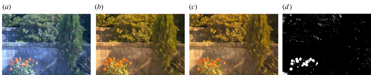
Figure 3. Images of scene 3 from figure 1 (a) under a 10 000 K illuminant, (b) under a 2900 K illuminant, (c) under a 2900 K illuminant but corrected for deviations in spatial cone-excitation ratios, and (d) with the locations of the largest tenth of the relative deviations marked in white.
