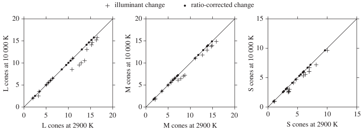
Figure 2. Estimated L, M, and S cone excitations from a small illustrative sample of points from scene 3 of figure 1 under a Planckian radiator illuminant with temperatures of 10 000 K and 2900 K (crosses) and with cone excitations corrected (solid circles) for deviations in spatial cone-excitation ratios. The fitted line is a linear regression. Axis scales have been adjusted for range after scaling cone excitations by the mean. See figure 3 for the images corresponding to these conditions.
