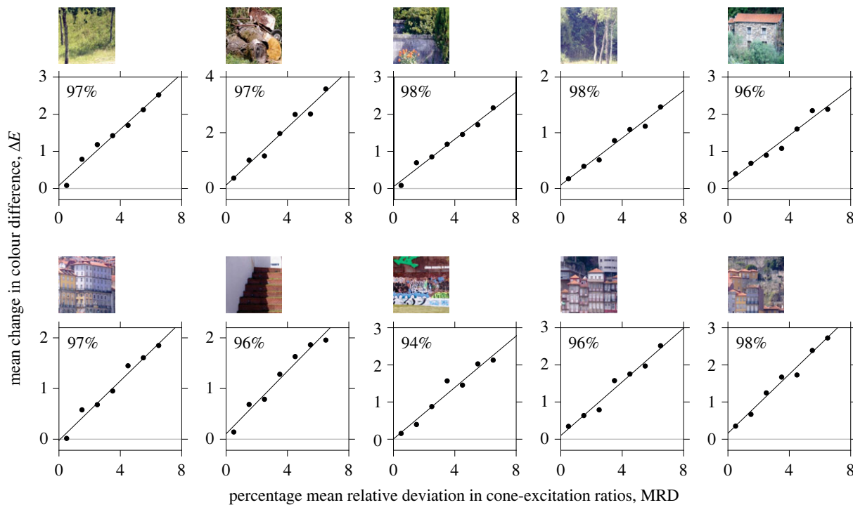
Figure 7. Changes in colour differences within scenes due to illuminant changes. Symbols show mean changes in estimated colour differences \Delta E in the approximately uniform colour space CAM02-UCS [43] corresponding to MRDs in spatial cone-excitation ratios. Fitted lines are linear regressions with adjusted goodness of fit R^2 shown in the top left of each panel. The horizontal grey line indicates zero change in colour differences.
