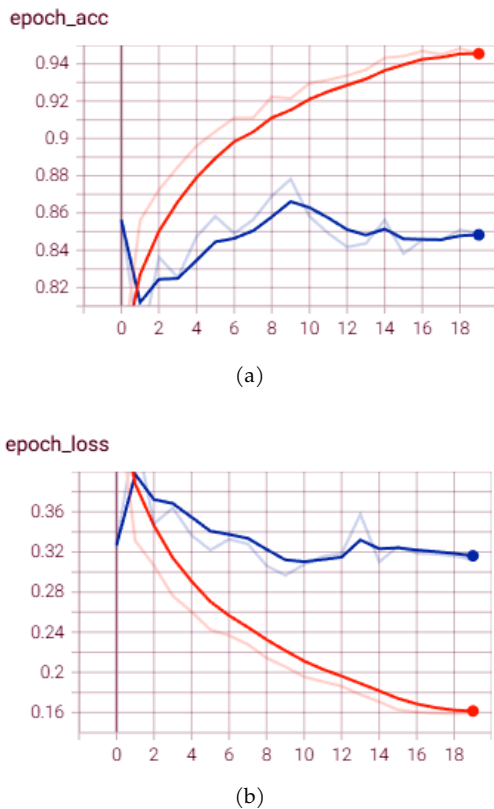
Fig. 14. a) Accuracy and b) loss curve for Xception. Training is represented by the orange line, and validation by the blue line.
