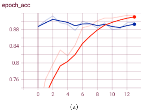
Fig. 10. a) Accuracy and b) loss curve for MobileNetV2. Training is represented by the orange line, and validation by the blue line.
