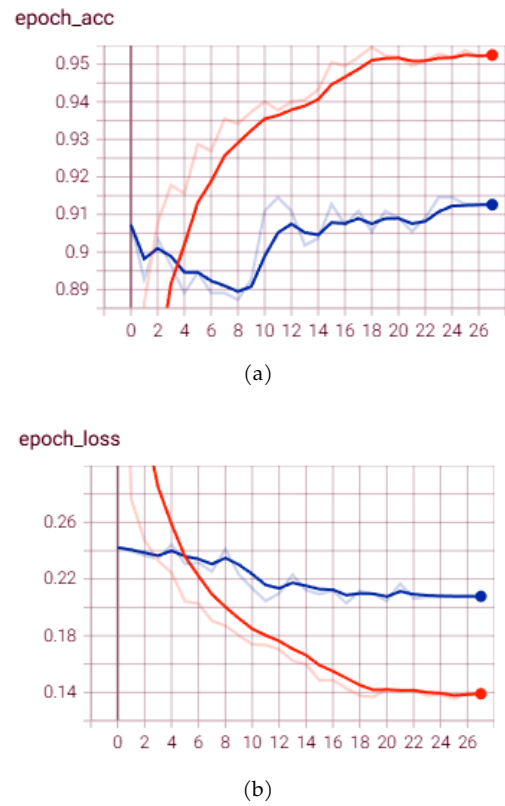
Fig. 6. a) Accuracy and b) loss curve for EfficientNetB0. Training is represented by the orange line, and validation by the blue line.
