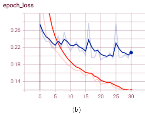
Fig. 7. a) Accuracy and b) loss curve for EfficientNetB1. Training is represented by the orange line, and validation by the blue line.
