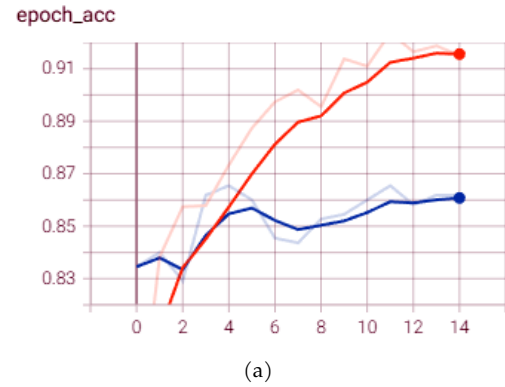
Fig. 12. a) Accuracy and b) loss curve for VGG16. Training is represented by the orange line, and validation by the blue line.
