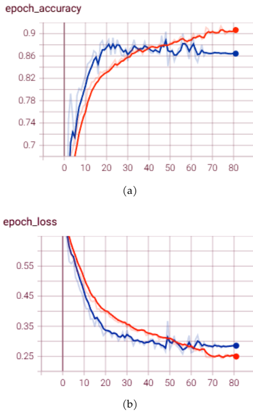
Fig. 5. a) Accuracy and b) loss curve for CNN. Training is represented by the orange line, and validation by the blue line.
