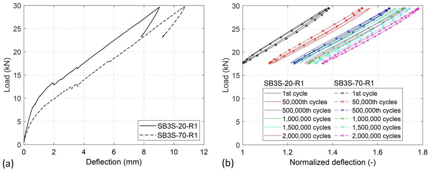
Fig. 9. Fatigue response of specimens SB3S-20-R1 and SB3S-70-R1: (a) Initial load-deflection response prior to cyclic loading, and (b) load versus normalized deflection curves during cyclic loading.
