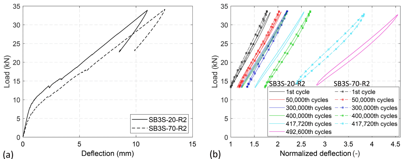
Fig. 10. Fatigue response of specimens SB3S-20-R2 and SB3S-70-R2: (a) Initial load-deflection response prior to cyclic loading, and (b) load versus normalized deflection curves during cyclic loading.
