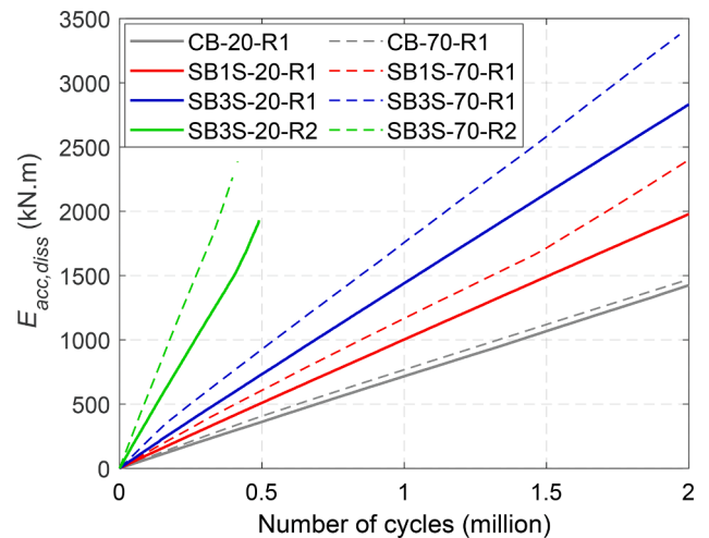
Fig. 17. Accumulated dissipated energy ( E_{acc,diss} ) versus number of cycles.
