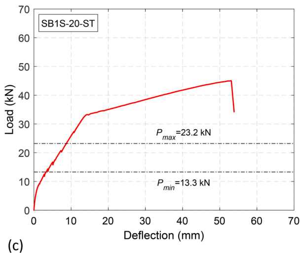
Fig. 6. Short-term load–deflection curves (Series 1): (a) Effect of strengthening ratio; (b), (c) and (d) definition of P_{max} and P_{min} .
