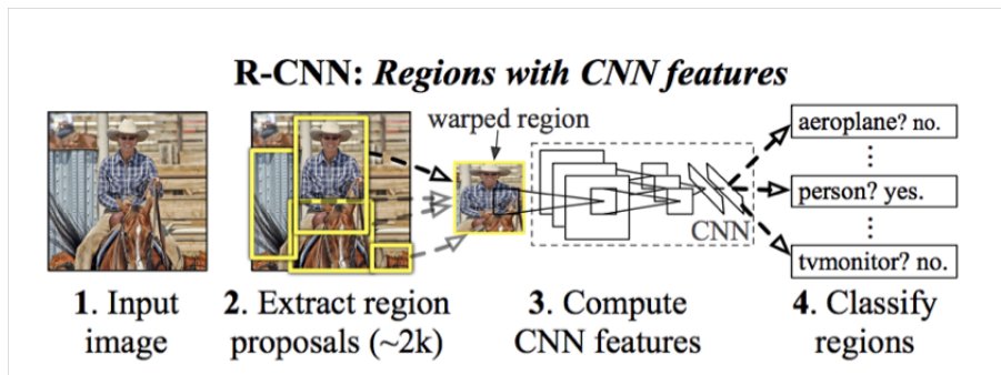
Figura 9: R-CNN: Regions with CNN features [23]
