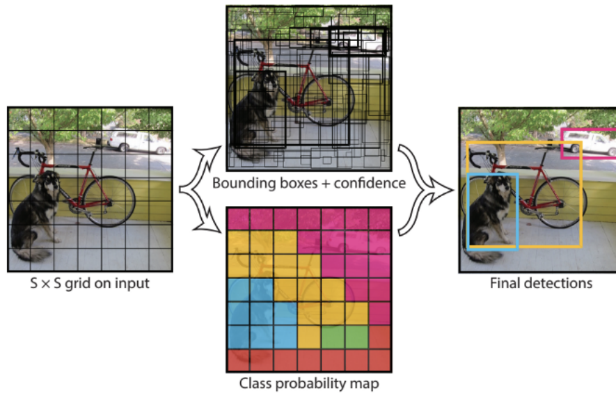
Figura 10: You Only Look Once (YOLO) [23]
