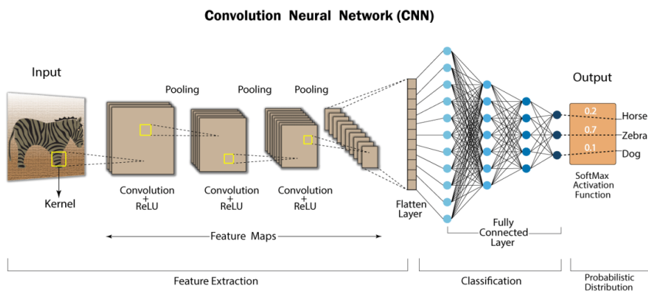
Figura 8: Convolutional Neural Network [57]
