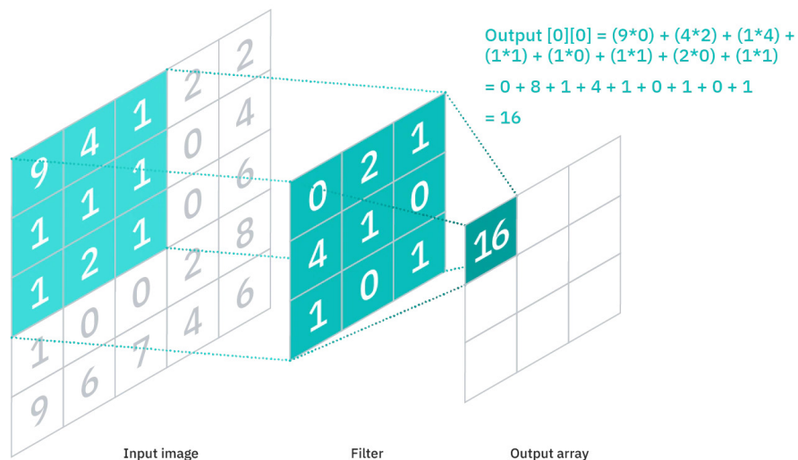
Figura 6: Convolutional layer [18]
