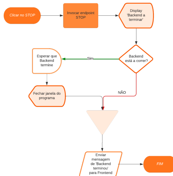
Figura 38: Fluxograma do endpoint STOP
