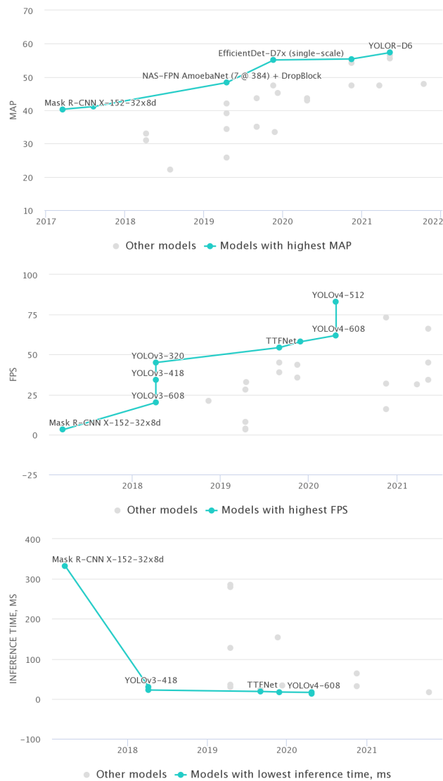
Figura 11: Real-Time Object Detection on COCO [1]
