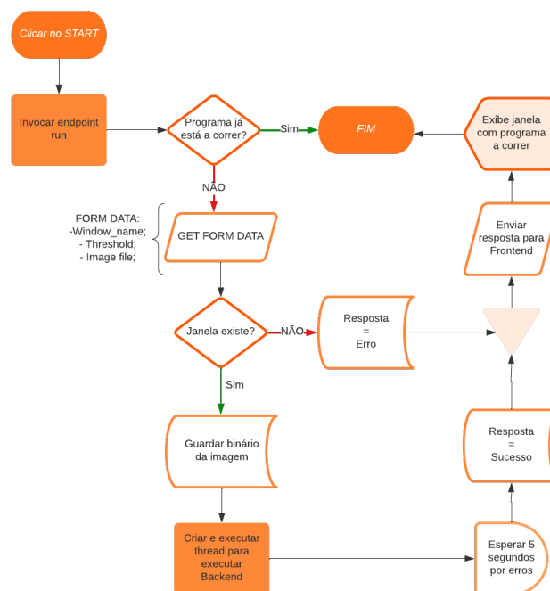
Figura 37: Fluxograma do endpoint RUN
