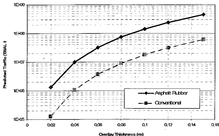
Figure 14 – Influence of bituminous mixture type in the overlay life (Sousa et al., 2005)
