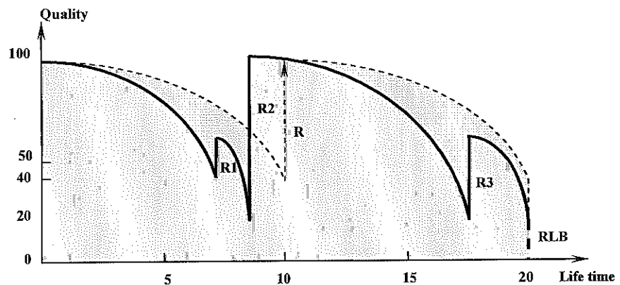
Figure 2 – The consequence of two rehabilitation strategies on the pavement life cycle
