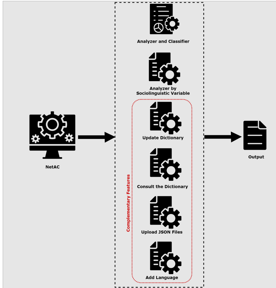
Fig. 3. NetAC Architecture
