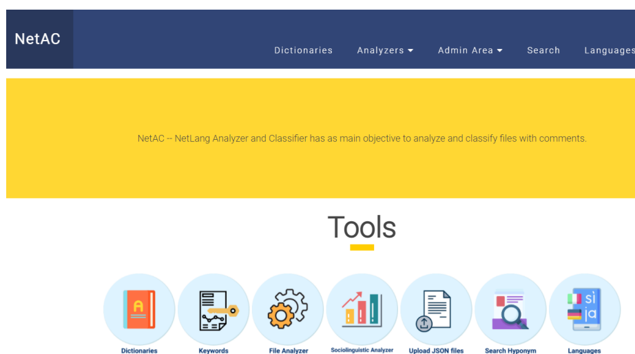
Fig. 6. NetAC – Homepage
