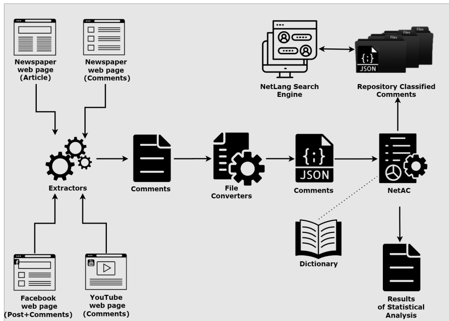
Fig. 2. NetLang Architecture
