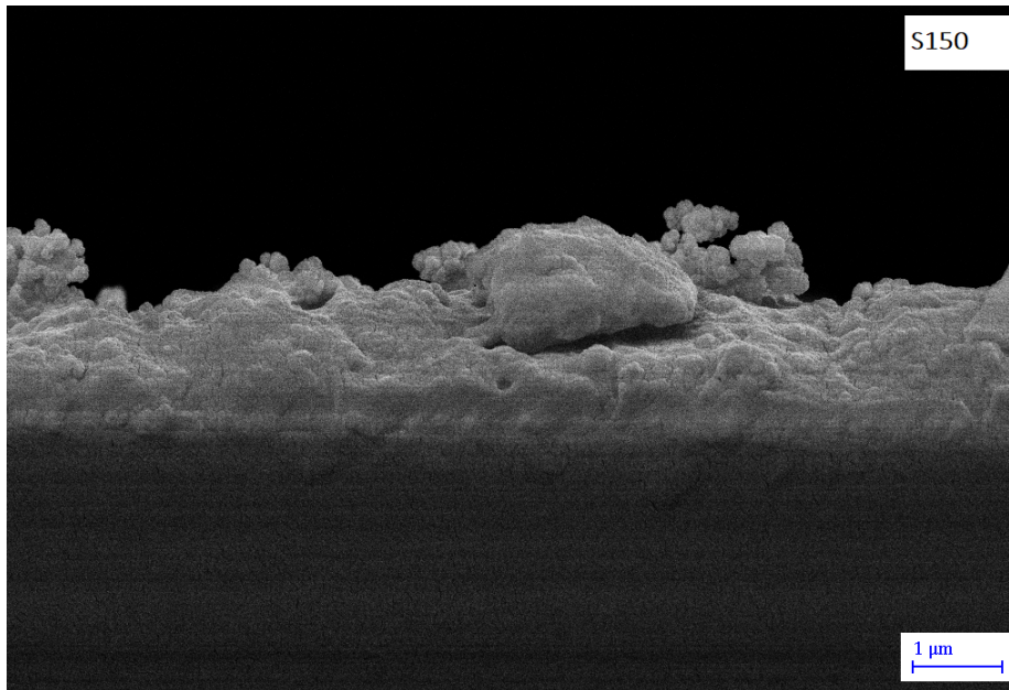
Figure S3: surface and cross section FESEM images of S150 sample.
