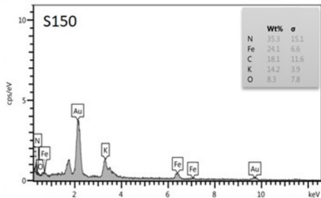
Figure S4: EDX analysis for S25, S100, and S150 samples.
