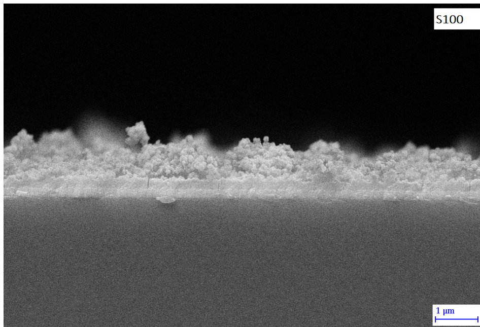
Figure S2: surface and cross section FESEM images of S100 sample.
