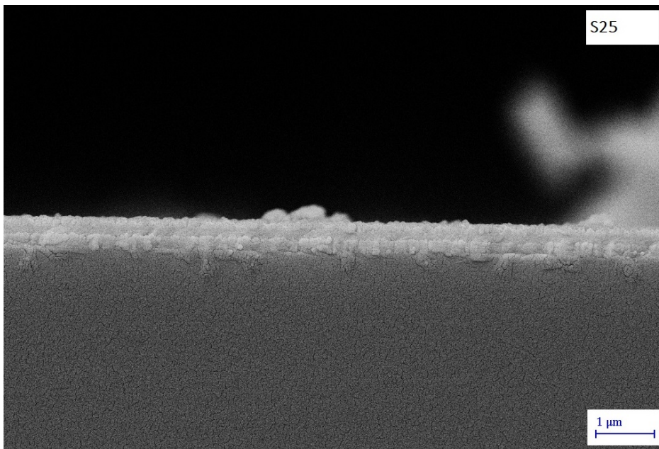
Figure S1: surface and cross section FESEM images of S25 sample.
