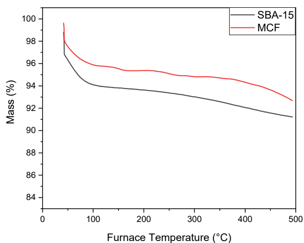
Figure 3. Thermogravimetric analysis (TGA) thermograms of the synthesized MCF and SBA-15 nanoparticles.
