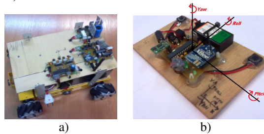
Fig. 3. a) Final aspect of the developed OMRP; b) Prototype of the remote control.
