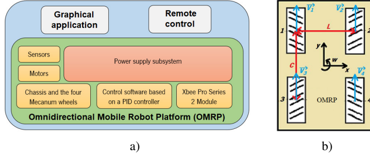
Fig. 1. a) Block diagram of the developed system; b) Schematic top view of the OMRP, clarifying the positions of the four Mecanum wheels and the referential used.
