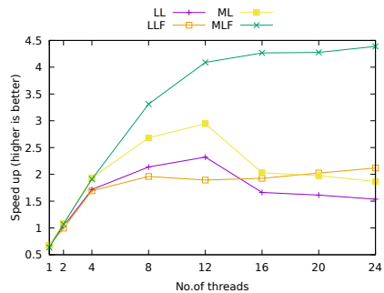
Figure 7: Breadth-first traversal on a graph using different queue implementations. LL: linearizable lock-based, LLF: linearizable lock-free, ML: mergeable lock-based, MLF: mergeable lock-free.
