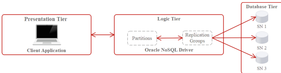
Fig. 1. Three-tier architecture
