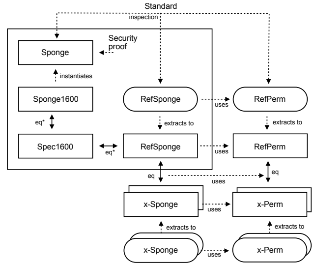
Figure 14: Equivalence proofs
