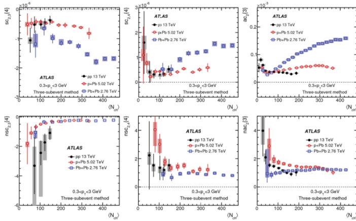
Fig. 2. The top row shows the \langle N_{ch} \rangle dependence of sc_{2,3}\{4\} (left column), sc_{2,4}\{4\} (middle column) and ac_2\{3\} (right column) obtained for pp collisions (solid circles), p+Pb collisions (open circles) and low-multiplicity Pb+Pb collisions (open squares) [9]. The bottom row shows the normalized versions of symmetric and asymmetric cumulants. The error bars and shaded boxes represent the statistical and systematic uncertainties, respectively.
