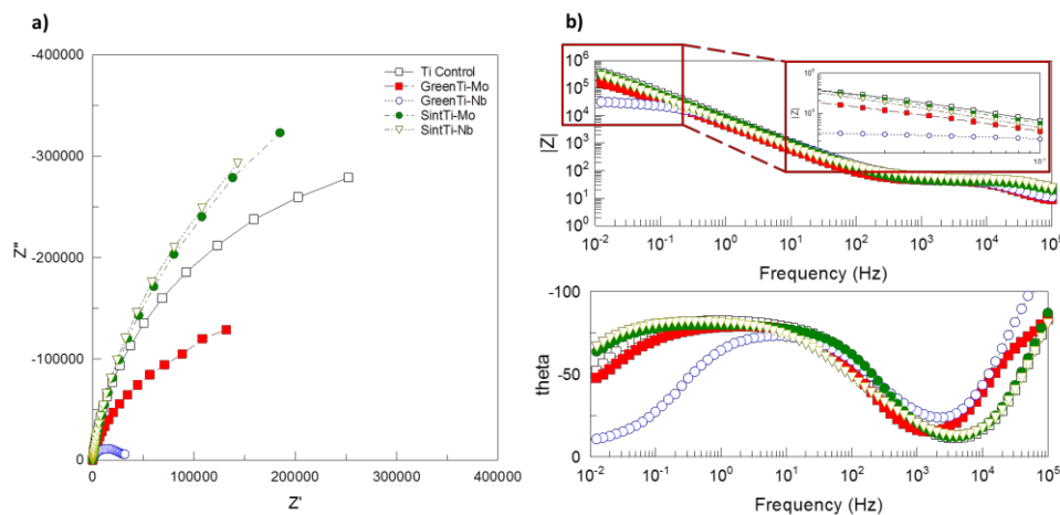
Figure 3. a) Nyquist and b) Bode plots obtained for the modified surfaces and control samples in 9 g/l NaCl solution
