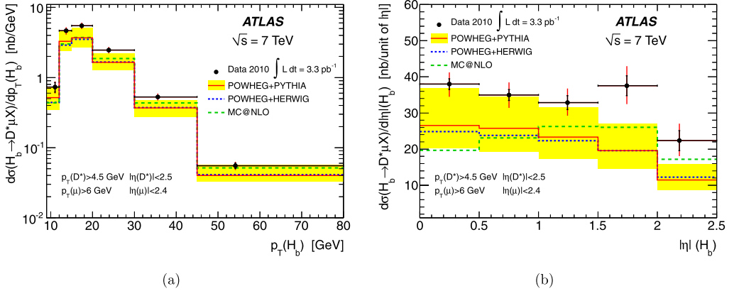
Fig. 2. Differential cross section for H_b \rightarrow D^{*+} \mu^- X production as a function of (a) p_T and (b) |\eta| of the b -hadron, in the fiducial kinematical region p_T(D^{*+}) > 4.5 GeV, p_T(\mu^-) > 6 GeV, |\eta(D^{*+})| < 2.5 and |\eta(\mu^-)| < 2.4 . The measurement is compared with the theoretical predictions, as described in the text. The inner error bars of the data points are statistical uncertainties, the outer are statistical + total systematic uncertainties.
