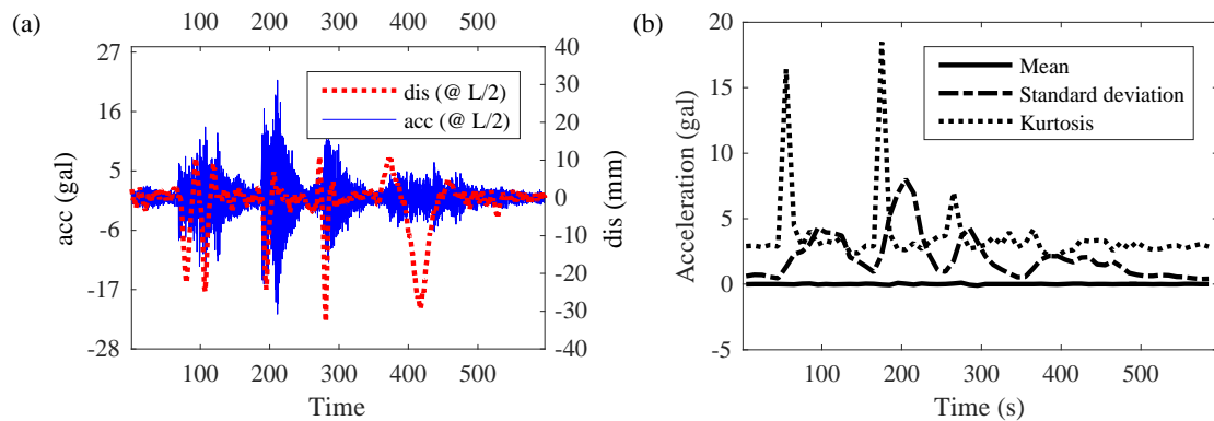
Fig. 13. (a) Measured displacement and acceleration at the center of mid span and (b) moving average, standard deviation and kurtosis of (a)
