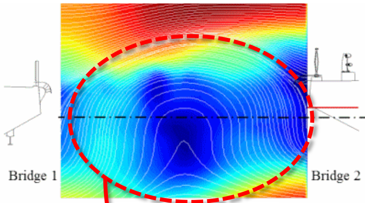
Parallel deck
