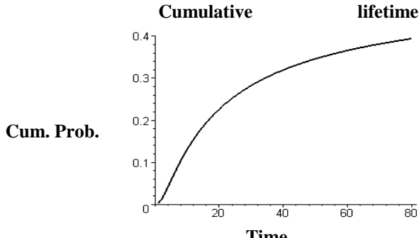
Fig. 5 Probability distribution of lifetime (superstructure) according to input statistical models given in Table 3.
