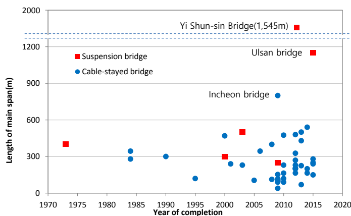
Fig. 1. Data of cable-supported bridges in Korea (Courtesy of TM-ENC)
