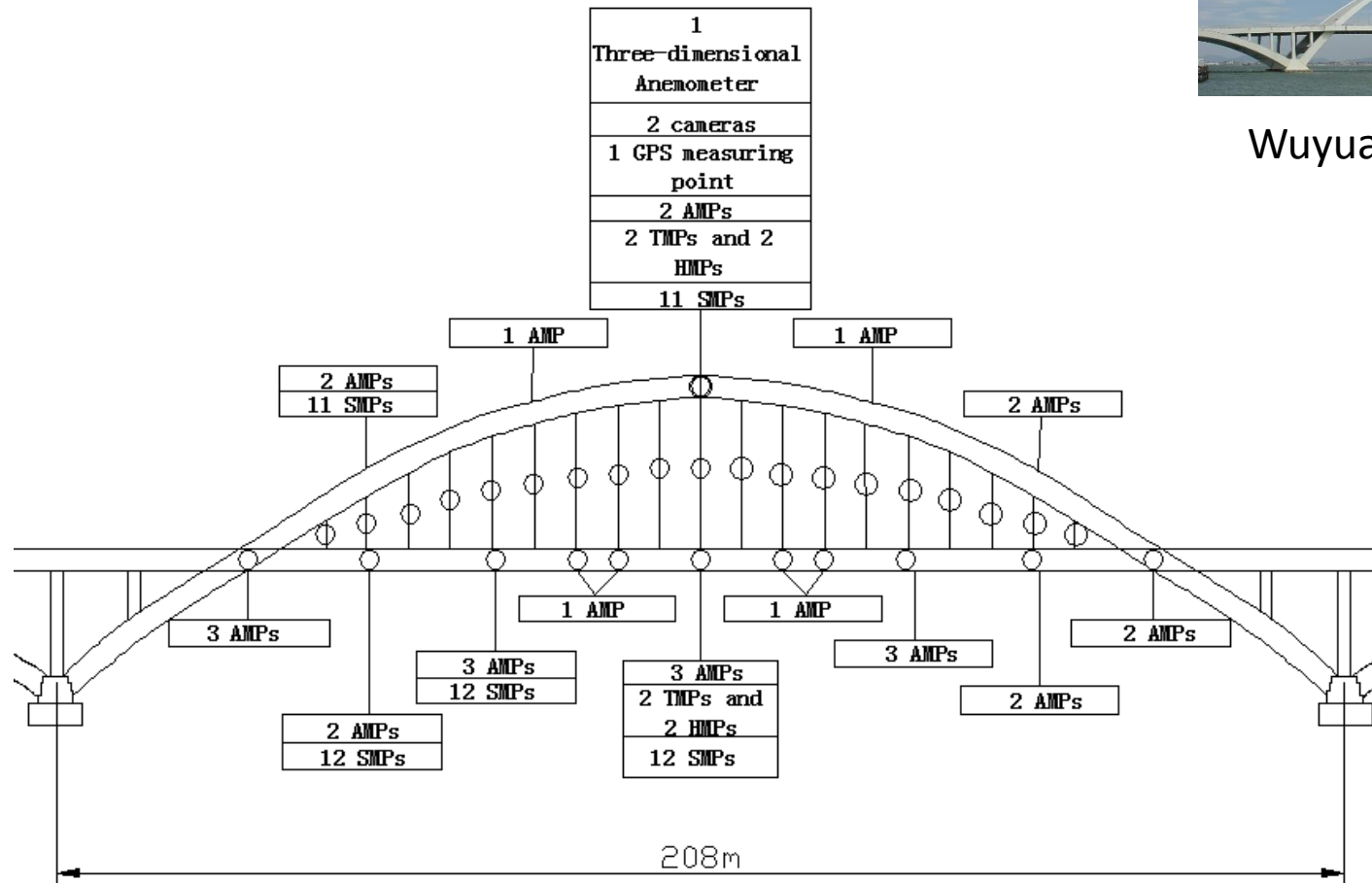
Sensor arrangement for Wuyuan Bridge
