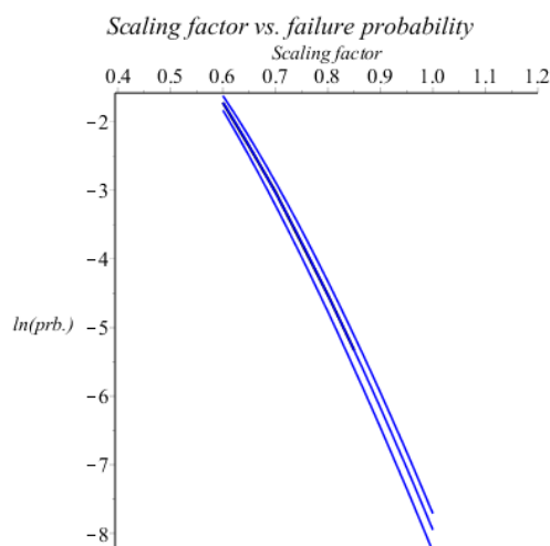
Figure 11. Failure probability as a function of the scaling parameter for system with 90 components subjected to chloride ingress. Failure probability at t = 60 years for the case that the surface concentrations for half the components are found to be smaller than 0.18%.
