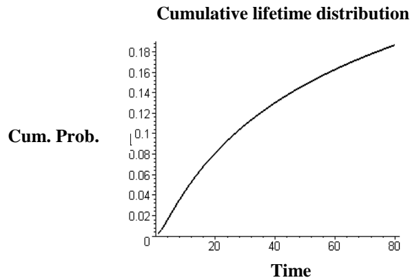
Fig. 7. Cumulative distribution function for chloride lifetime. Alpha-parameter which defines variation of diffusion coefficient with time is represented by a lognormal distribution with mean value 0.4 and a standard deviation of 0.1
