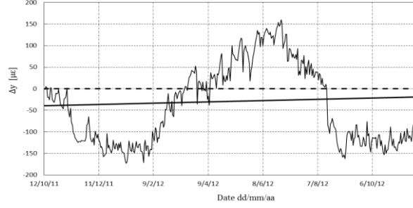
Fig. 3. Relative strain of cable ITN and interpolating lines.
