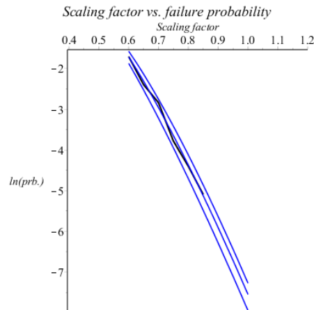
Figure 10. Failure probability as a function of the scaling parameter for system with 90 components subjected to chloride ingress. Failure probability at t = 60 years for the case that the surface concentrations for half the components are found to be smaller than 0.196%.
