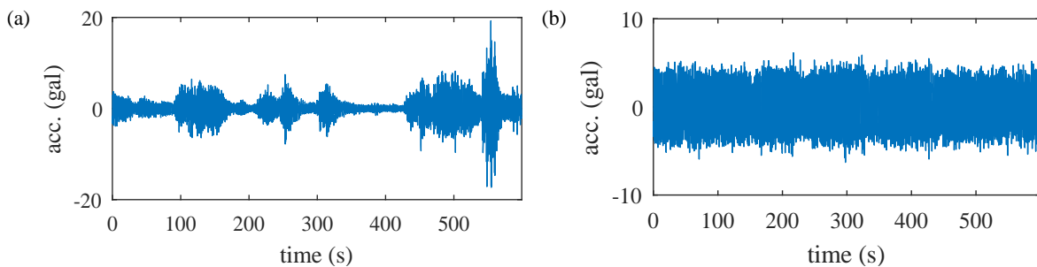
Fig. 14. (a) Measured acceleration and (b) approximated stationary acceleration
