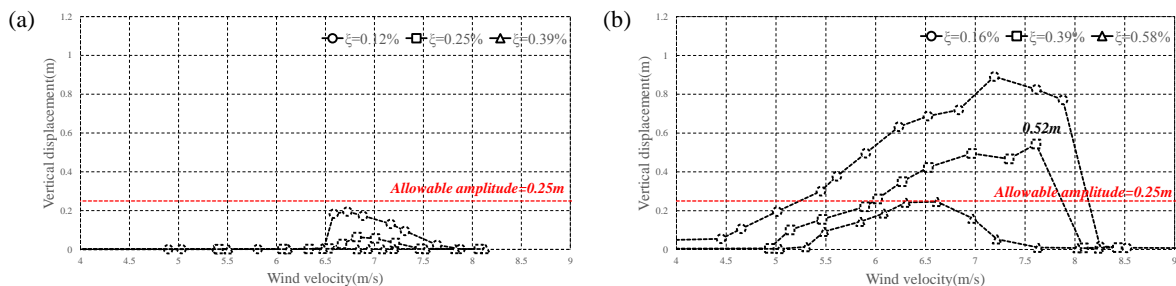
Fig. 12. Amplitude of VIV with (a) As-built guardrails, (b) covered guardrails temporarily
