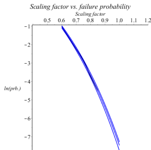
Figure 9. Failure probability as a function of the scaling parameter at a time of t = 60 years without any additional information (from monitoring or inspection) being available.
