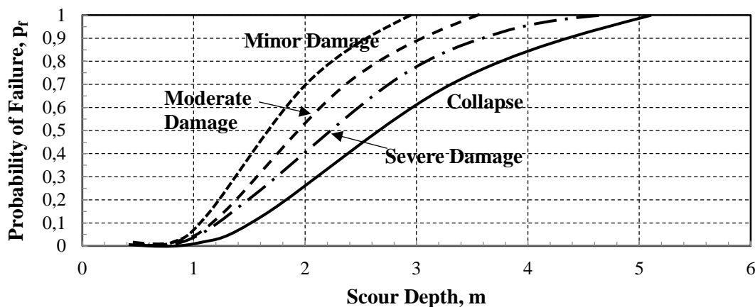
Figure 3 Development of fragility curves for the effect of scour on bridges
