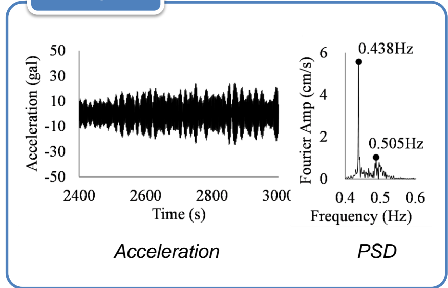
Bridge 1
