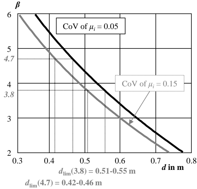
Fig. 2. Variation of reliability index \beta with snow depth d and limiting values d_{lim} for the selected target levels.
