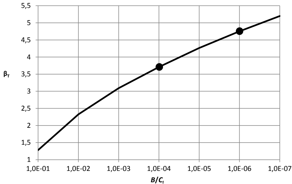
Fig. 3. Variation of the target reliability index \beta_T with the ratio B/C_f
