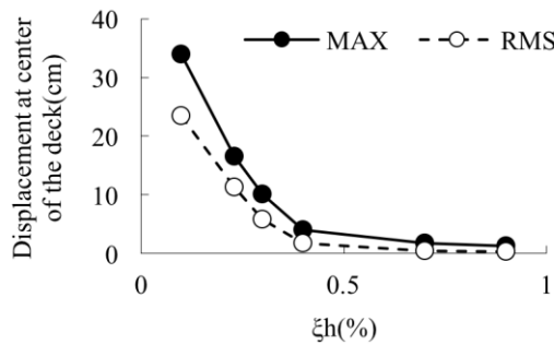
Fig. 8. Amplitude of VIV for set-up damping ratio in wind tunnel
