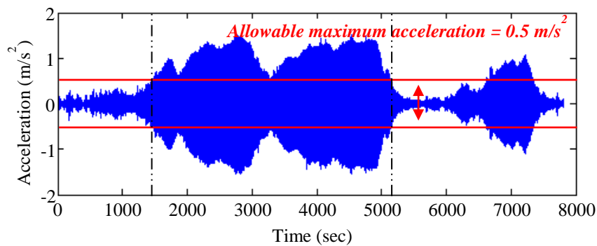
Fig. 5. Vertical acceleration of the deck in Bridge 2 at the center of main span
