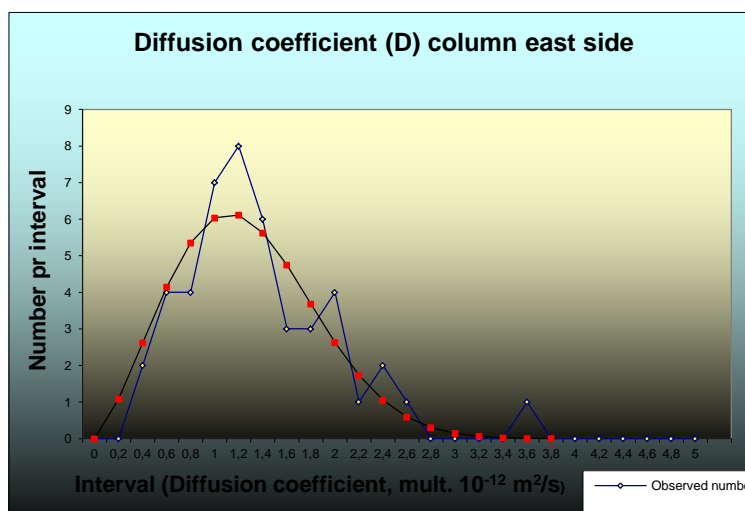
Fig. 3. Observed versus predicted number of samples for the diffusion coefficient within each interval, east side of columns. Theoretical model is based on regression curve in Figure 2.
