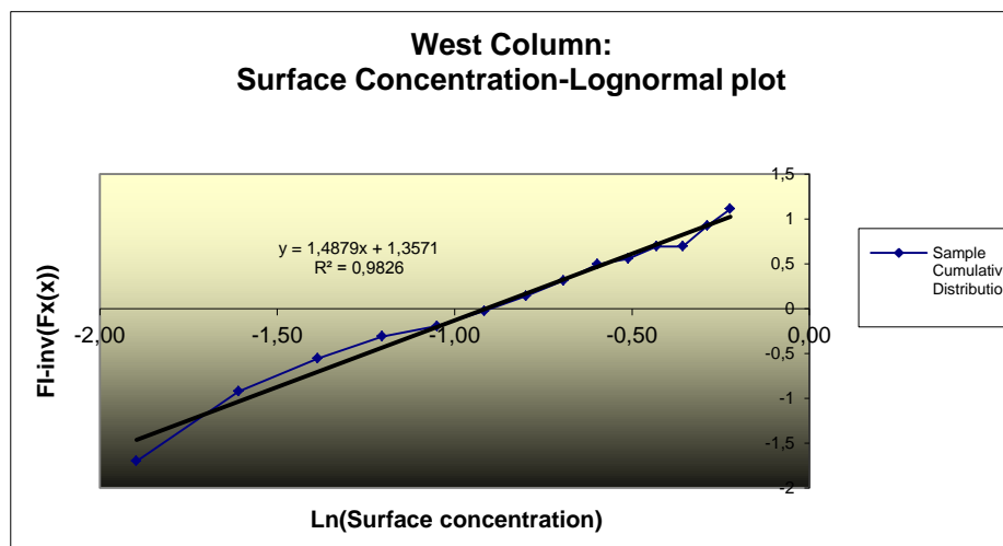
Fig. 4. Cumulative distributions for measured surface concentration plotted in lognormal scale, and resulting fitted lognormal model. West side of columns.
