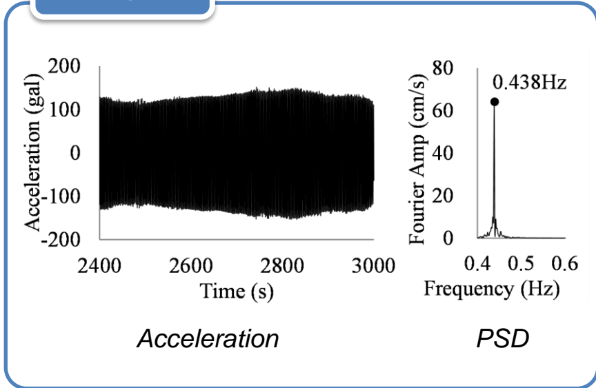
Bridge 2
