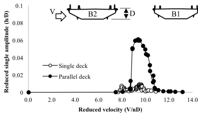
Fig. 6. Amplitude of VIVs in both a single deck and parallel decks
