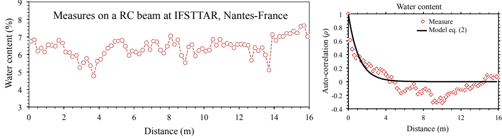
Fig. 3. a- Experimental trajectories of water content; b- auto-correlation data and fitted ACFs for water content in a RC beam (IFSTTAR, Nantes, France)
