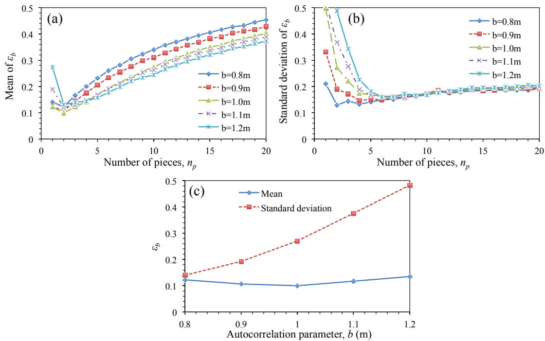
Fig. 2. Sensitivity of \varepsilon_b for: a - the mean of \varepsilon_b ; b - the standard deviation of \varepsilon_b c - the mean and standard deviation of \varepsilon_b for n_p=2 ( N_s=200 , L=100m )
