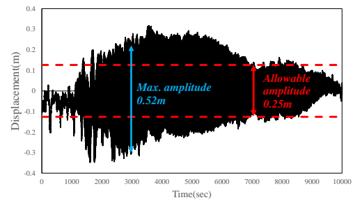
Fig. 11. Time history of VIV
