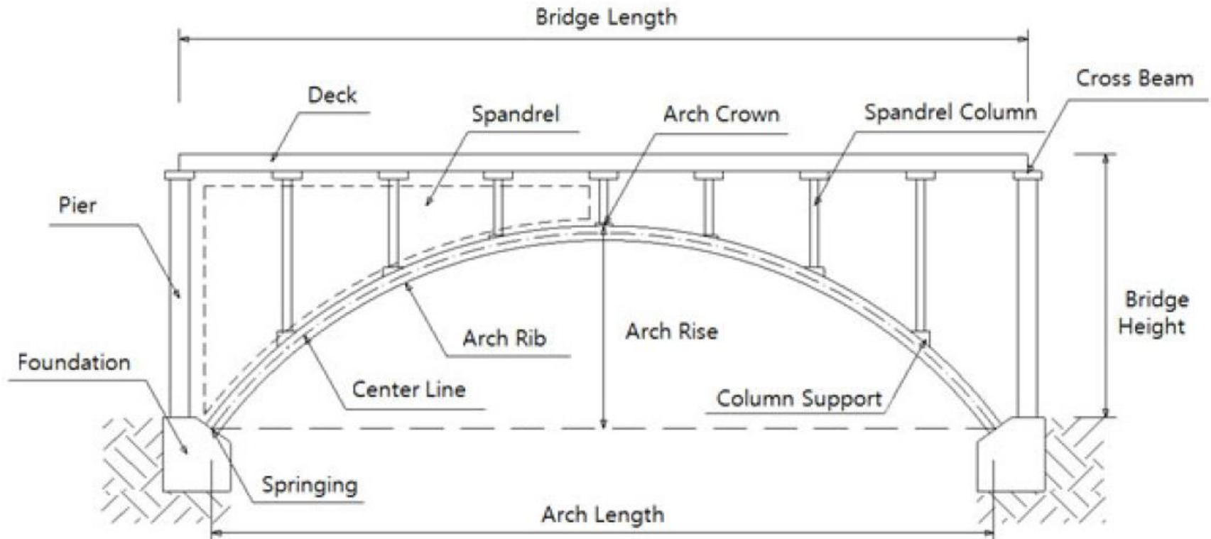
Outline of Arch Bridge, M. Han et. al., 2016
