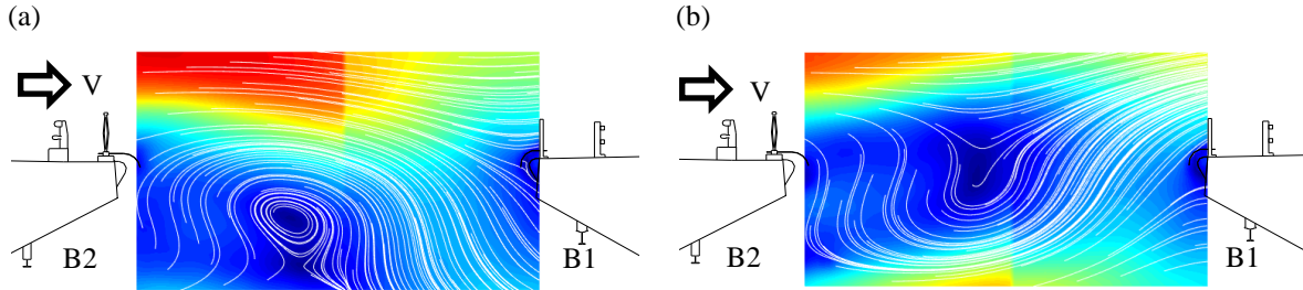
Fig. 7. Phase-averaged flow streams at the phase of (a) \pi/2 , (b) 3\pi/2
