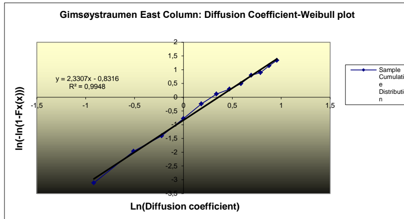
Fig. 2. Comparison between sample distribution function and fitted Weibull distribution for the diffusion coefficient, east side of columns.
