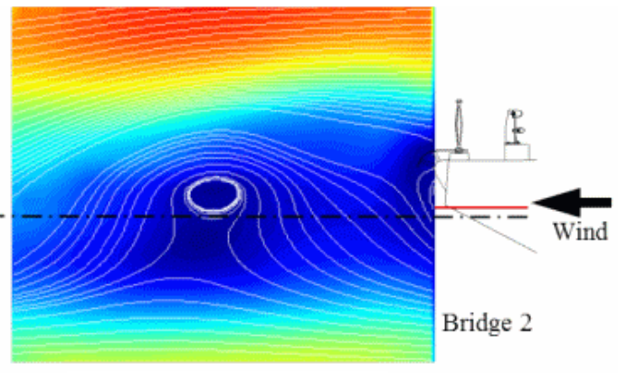
Single deck
