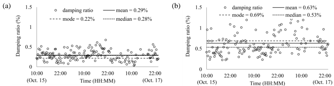
Fig. 9. Estimated damping ratio of (a) Bridge 2 and (b) Bridge 1
