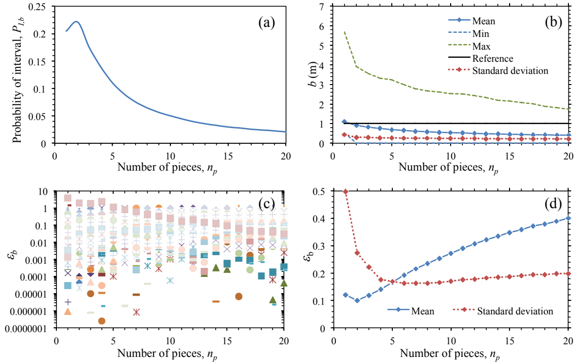
Fig. 1. Effect of number of pieces n_p on: a - the probability of interval P_{I,b} ; b - the estimated values of b c - the distribution of \varepsilon_b ; d - the mean and standard deviation of \varepsilon_b ( N_s=200 , L=100\text{m} and \Delta=10\% )
