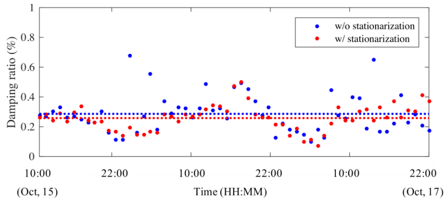
Fig. 15. Estimated damping ratio
