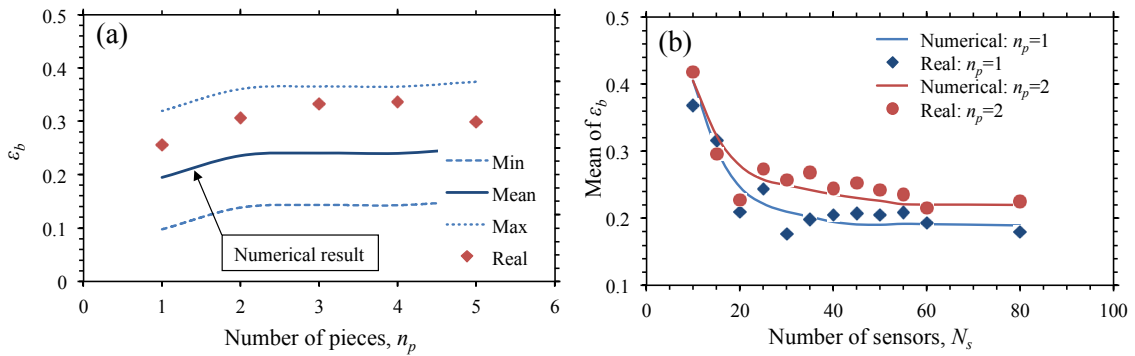
Fig. 4. Comparison between simulated results and real inspection values in the case of water content (RC beam, L=16 m, IDT=0.4\text{m} ):
