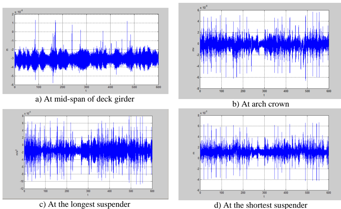
Fig. 5 Strain time history at some measuring points
