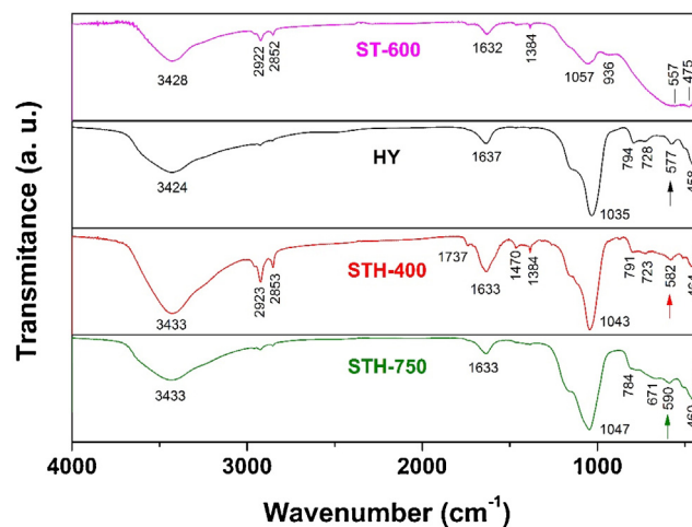
Fig. 2. FTIR spectrum of HY zeolite compared to the spectra of other composites. The arrows indicate the wavenumber used to calculate the Si/Al ratio by utilizing Eq. (1).
