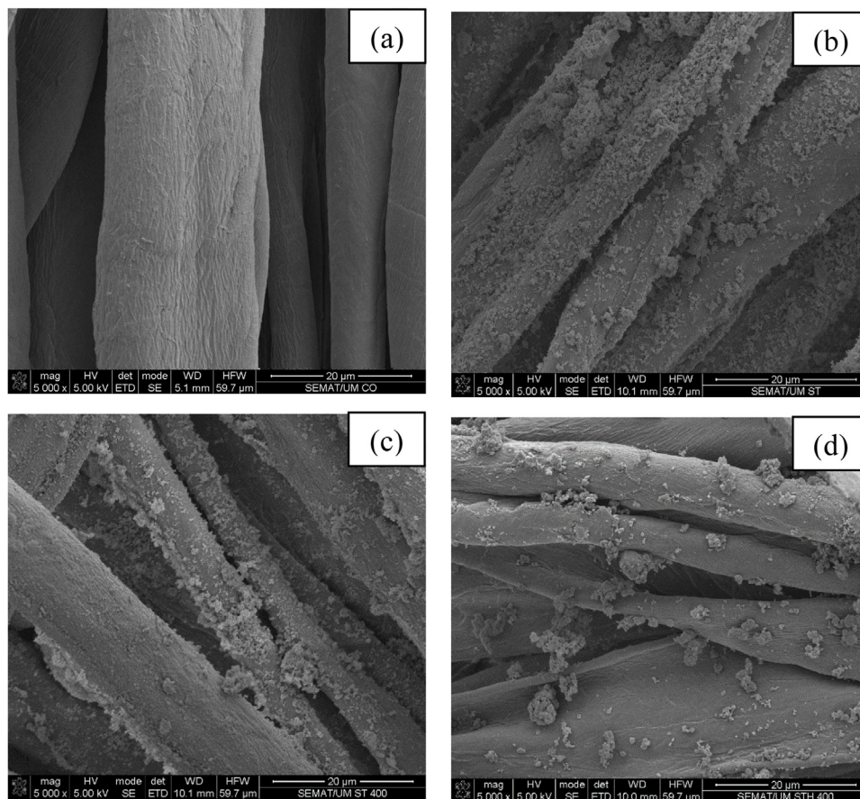
Fig. 5. SEM micrographs of cotton pristine cotton (a) and cotton textiles coated with (b) ST, (c) ST-400 and (d) STH-400 photocatalysts at a magnification of 5000 \times .
