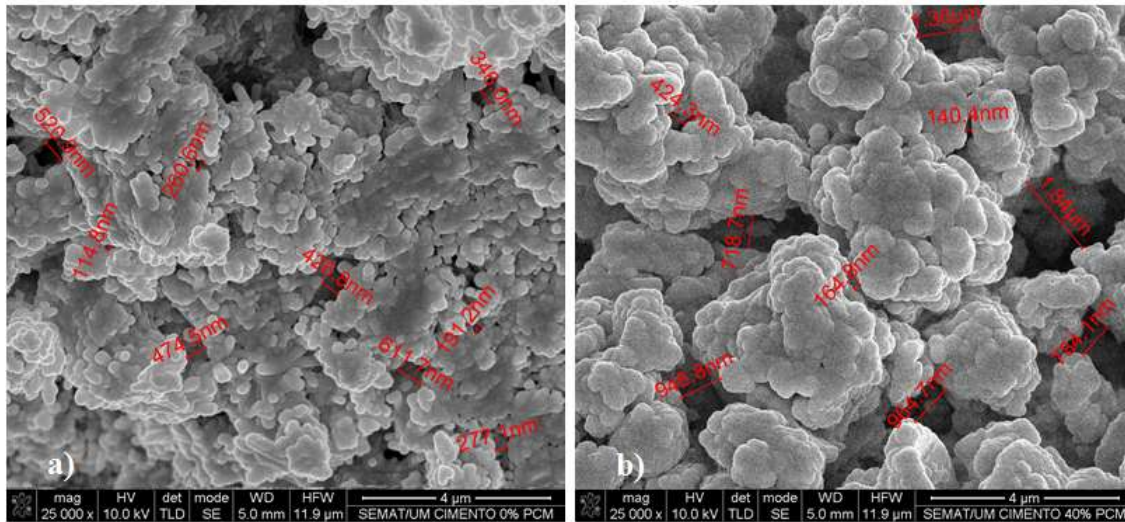
Fig. 6 - Microscope observation of cement based mortars, enlargement of 25000x: a) Mortar without incorporation of PCM microcapsules; b) Mortar with incorporation of 40% of PCM microcapsules and 1% of fibers.
