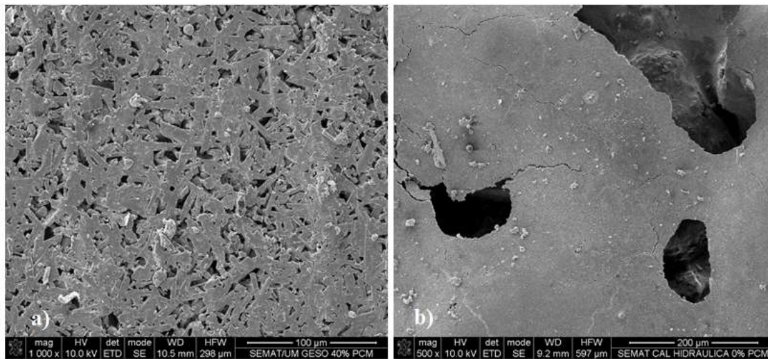
Fig. 9 - Surface of mortars: a) Gypsum based mortar, enlargement of 1000x, b) Hydraulic lime based mortar, enlargement of 500x.
