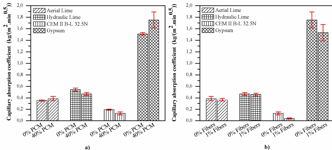
Fig. 7 - Capillary absorption coefficient: a) Variation with PCM content, b) Variation with fibers content.
