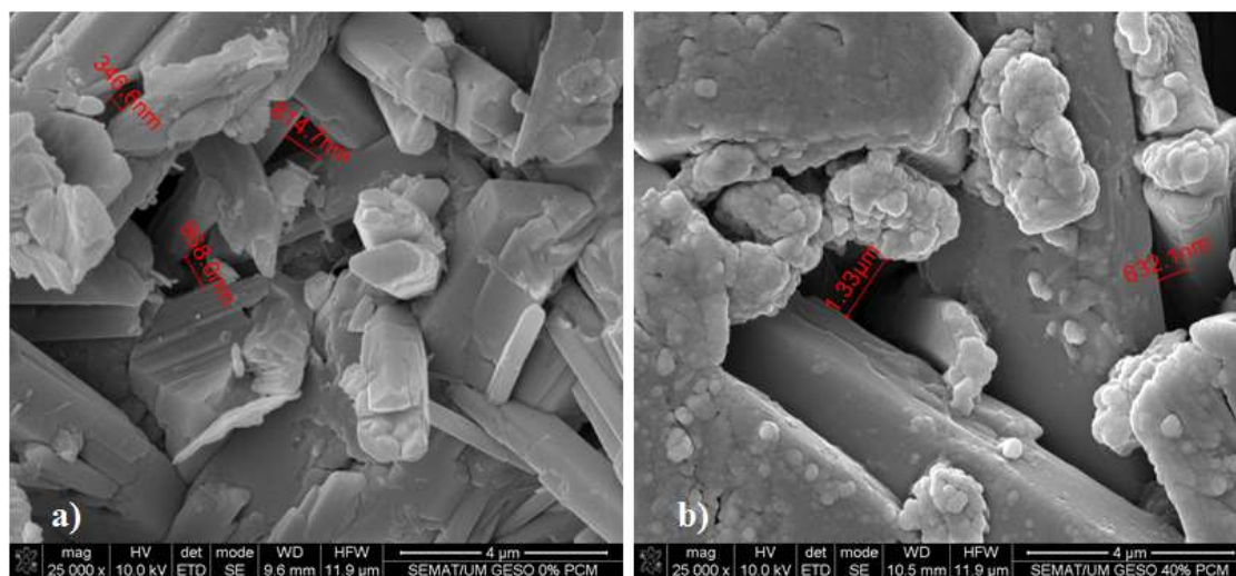
Fig. 5 - Microscope observation of gypsum based mortars, enlargement of 25000x: a) Mortar without incorporation of PCM microcapsules; b) Mortar with incorporation of 40% of PCM microcapsules and 1% of fibers.
