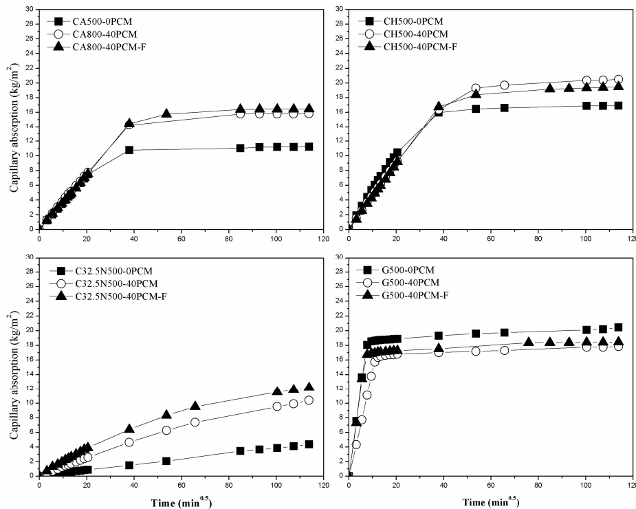
Fig. 2 - Water absorption by capillarity.
