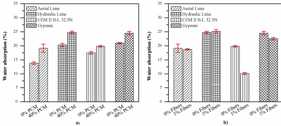
Fig. 8 - Water absorption of the mortars: a) Variation with PCM content, b) Variation with fibers content.
