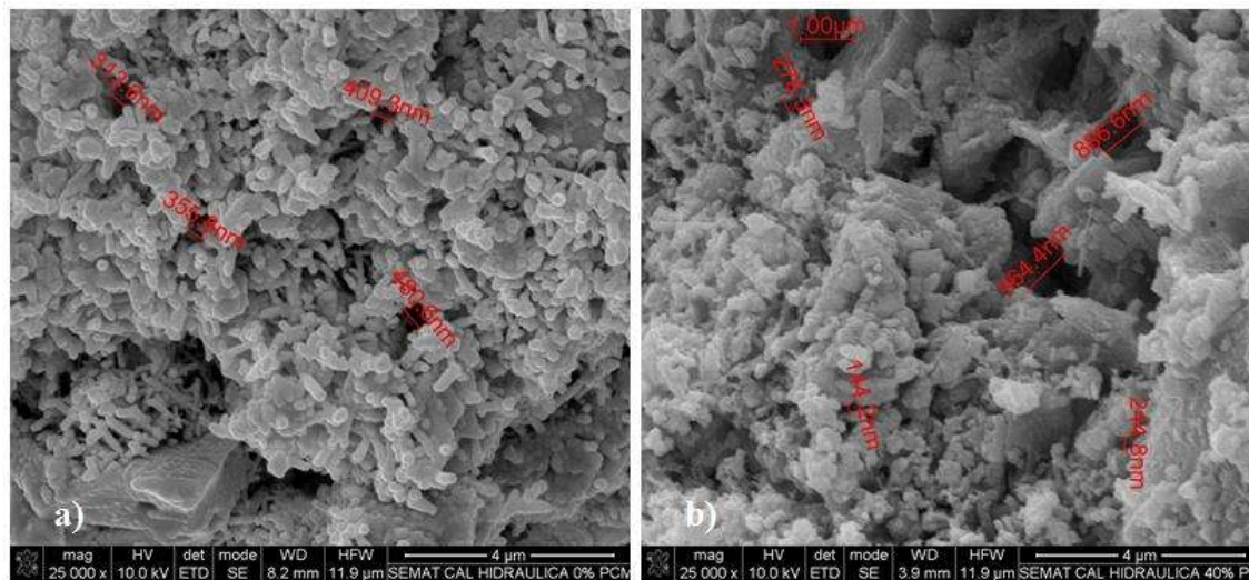
Fig. 4 - Microscope observation of hydraulic lime based mortars, enlargement of 25000x: a) Mortar without incorporation of PCM microcapsules; b) Mortar with incorporation of 40% of PCM microcapsules and 1% of fibers.
