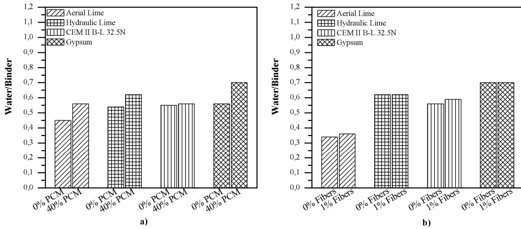
Fig. 1 - Water/Binder ratio: a) Variation with PCM content, b) Variation with fibers content.
