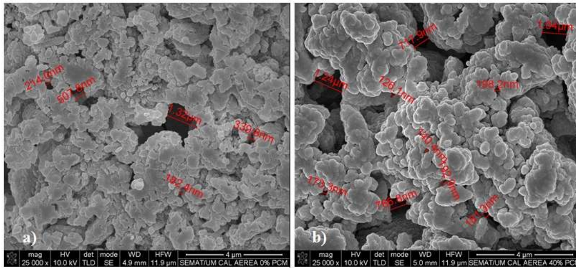
Fig. 3 - Microscope observation of aerial lime based mortars, enlargement of 25000x: a) Mortar without incorporation of PCM microcapsules; b) Mortar with incorporation of 40% of PCM microcapsules and 1% of fibers.
