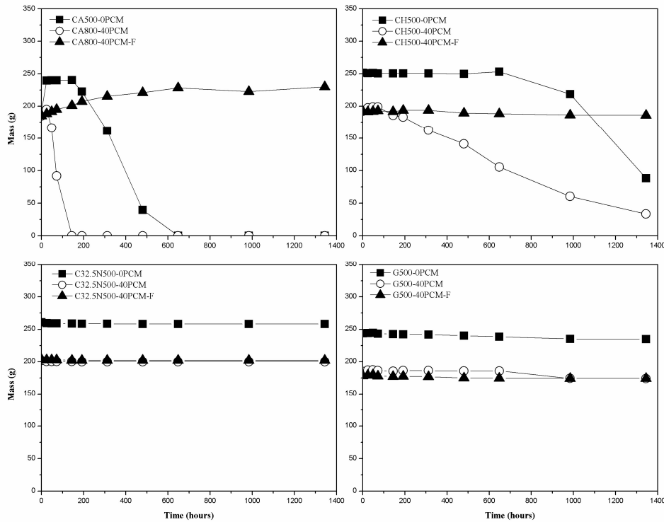
Fig. 10 - Behavior of the mortars to freeze-thaw cycles.
