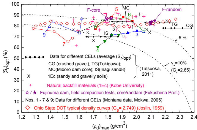
Figure 8: (S_r)_{opt} - (\rho_d)_{max} relations from a wide variety of laboratory compaction test data (Tatsuoka, 2015).
