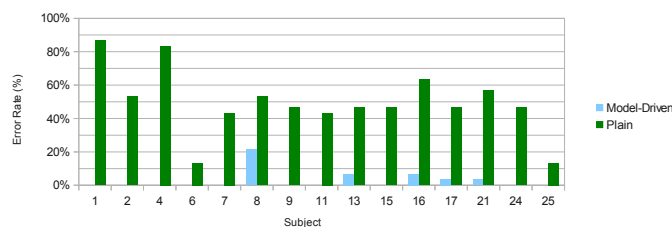
Fig. 13: Error rate in the budget spreadsheet.
