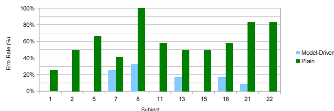
Fig. 14: Error rate in the payments spreadsheet.
