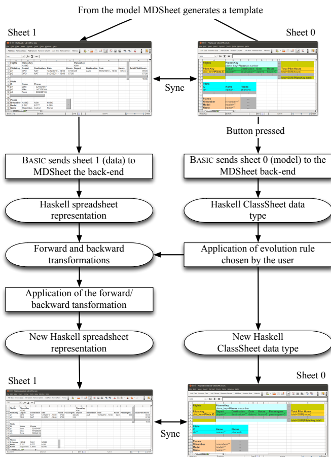
Fig. 10: Model-driven spreadsheet development environment.
