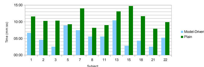
Fig. 12: Time used to perform the tasks on the payments spreadsheet.
