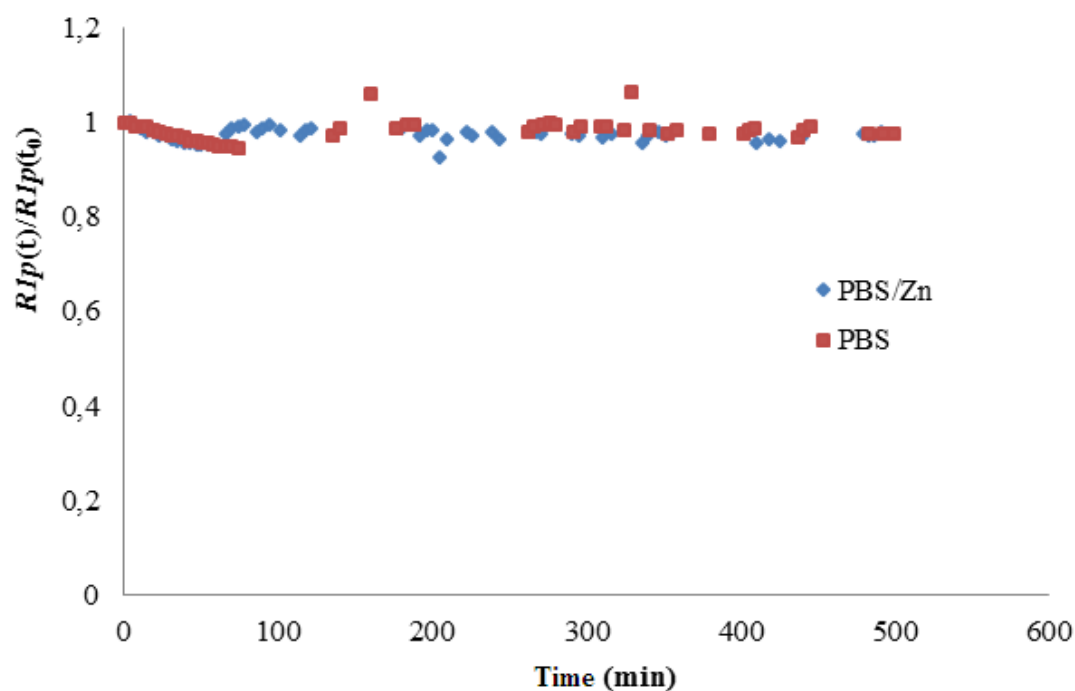
Figure SI12. Time evolution of the relative water proton paramagnetic relaxation rate R_{1p}(t)/R_{1p}(0) (20 MHz, 25 °C) for a solution of GdL_2@AuNPs (1.30 mM in PBS 10 mM, pH 7.1) (■) and following addition of 0.75 mM ZnCl_2 (◆).
