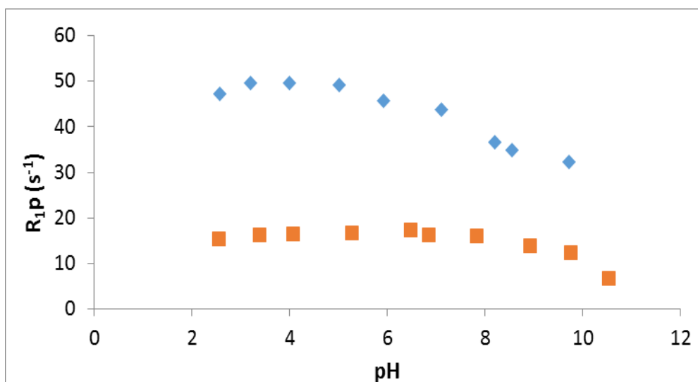
Figure SI10. pH dependence of the paramagnetic water proton relaxation rate for GdL 1 @AuNPs (20 MHz, 25 °C, 0.53 mM, (■)) and for GdL 2 @AuNPs (20 MHz, 25 °C, 1.30 mM (◆)).
