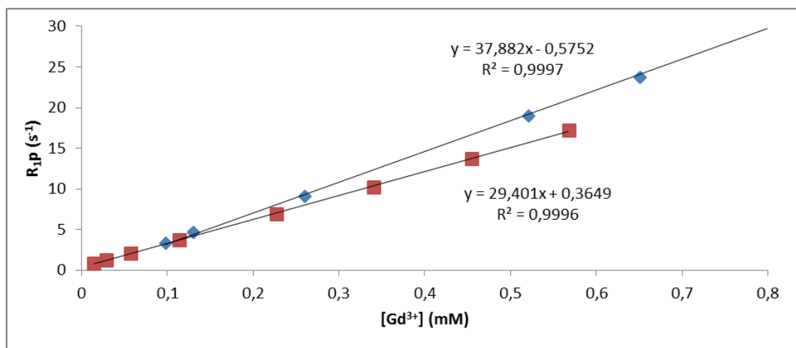
Figure SI9. Concentration dependence of the paramagnetic water proton relaxation rate R_{1p} ( R_{1p} = R_{1obs} - R_{1d} ) for GdL 1 @AuNPs (■) and GdL 2 @AuNPs (◆) (20 MHz, 25 °C, pH 7.1).
