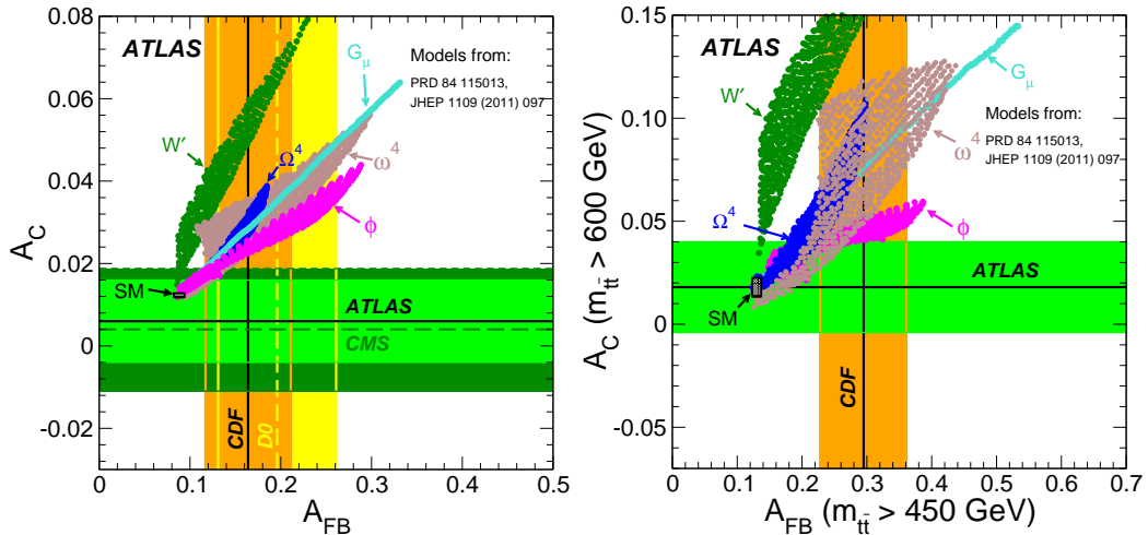
Figure 3. Measured forward-backward asymmetries A_{FB} at Tevatron and charge asymmetries A_C at LHC, compared with the SM predictions (black box) as well as predictions incorporating various potential new physics contributions (as described in the figure) [8, 60]. In both plots, where present, the horizontal bands and lines correspond to the ATLAS (light green) and CMS (dark green) measurements, while the vertical ones correspond to the CDF (orange) and D0 (yellow) measurements. The inclusive A_C measurements are reported in the left plot. In the right plot a comparison is reported between the A_{FB} measurement by CDF for m_{t\bar{t}} > 450 GeV and the A_C measurement for m_{t\bar{t}} > 600 GeV.
