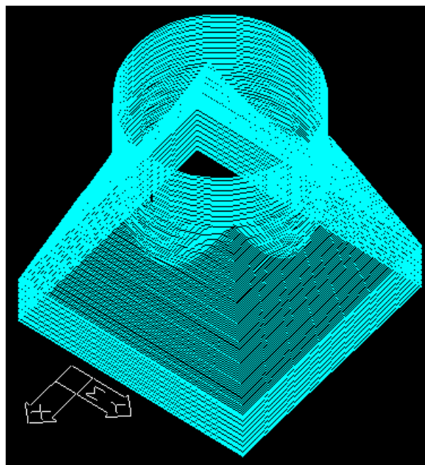
Figure 2 - Slices Generated for this shape
