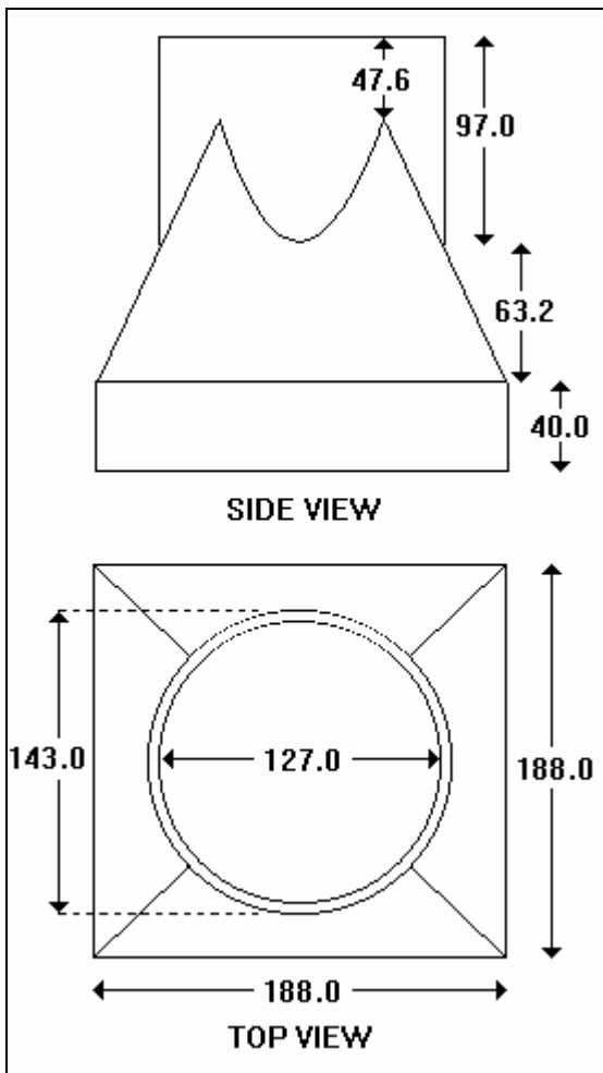
Figure 3 - Side and top view of the shape with dimensions in millimetres
