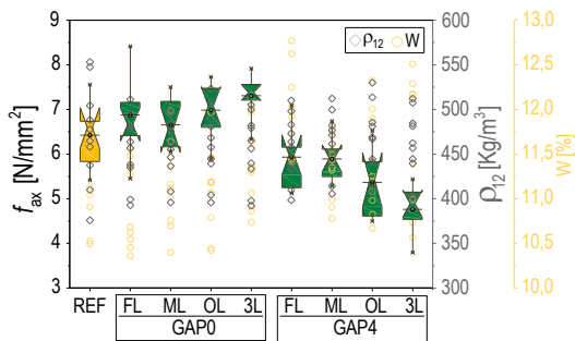
Fig. 5 – Results obtained by all nine test configurations with 12% of moisture content, concerning f_{ax} , \rho_{12} , and w .
