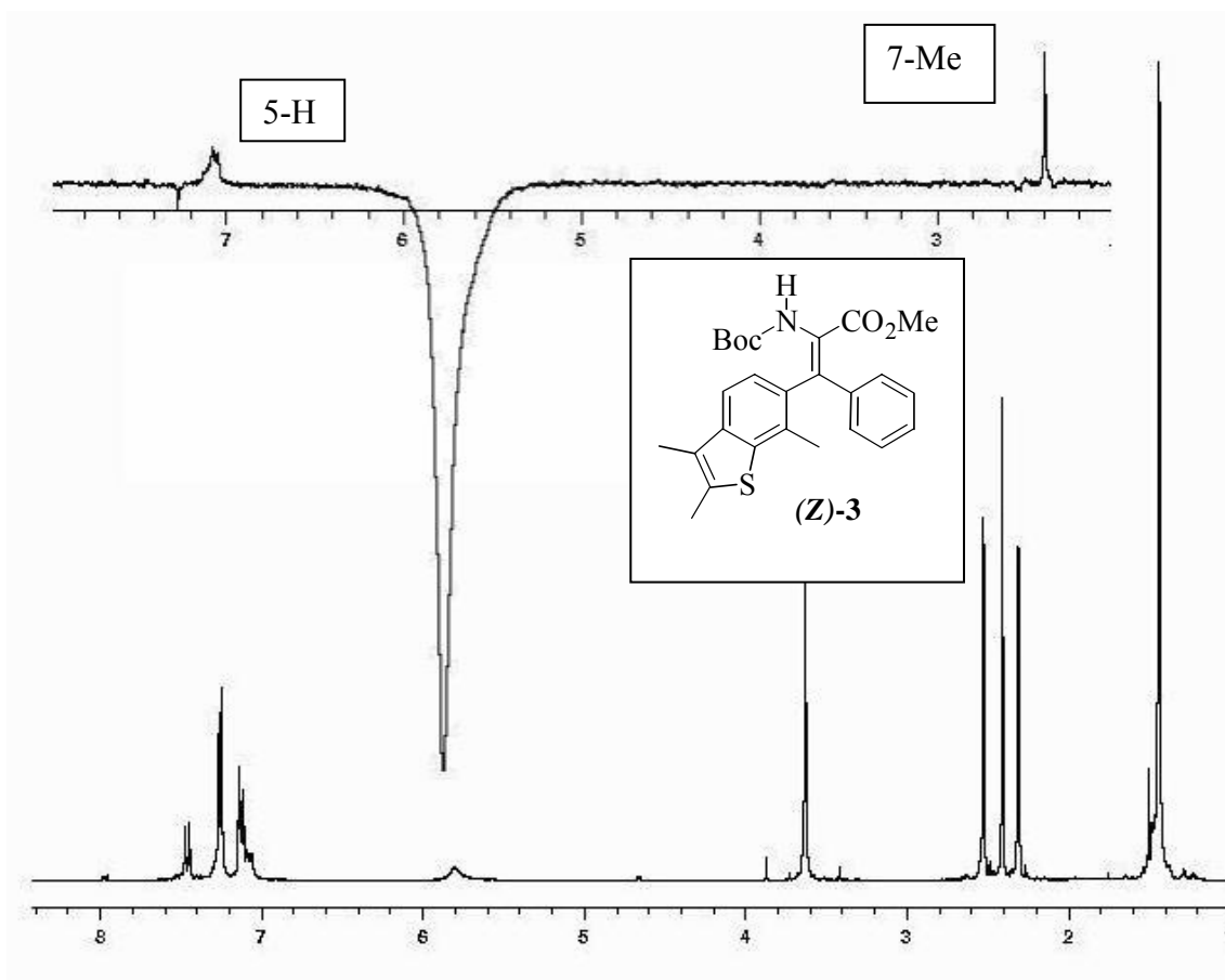
Fig. 1- ^1\text{H-NMR} ( \text{CDCl}_3 ) spectrum and NOE difference experiment irradiating the \alpha\text{NH} of compound (Z)-3.
