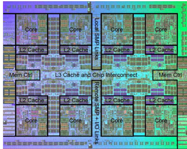
Figure 2.2: Schematic representation on a die of a CPU chip (image retrieved from www.anandtech.com ).
