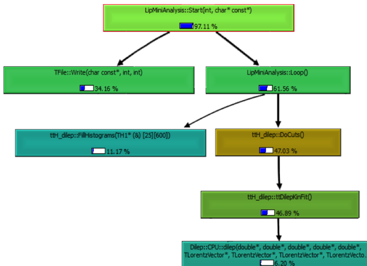
Figure 3.2: Callgraph for the t\bar{t}H_{dilep} application on the compute-711 node.
