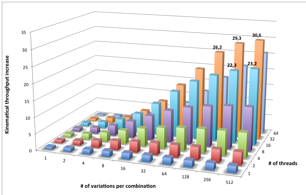
Figure 4.9: Kinematical reconstruction throughput for various values of variations and threads.
