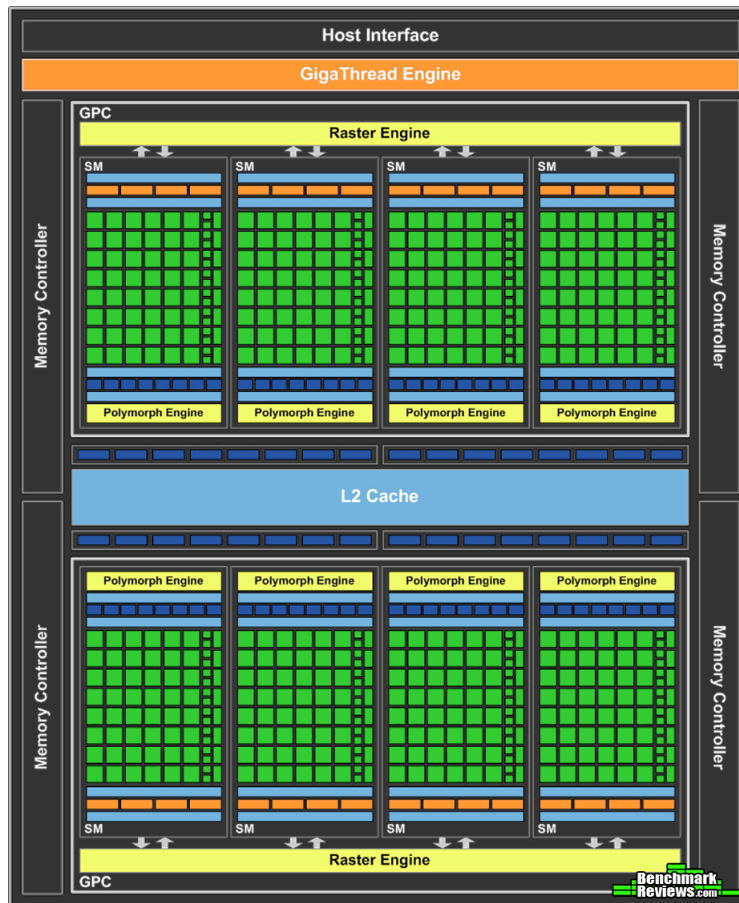
Figure 2.4: Schematic representation of the NVidia Fermi architecture (image retrieved from www.benchmarkreviews.com ).
