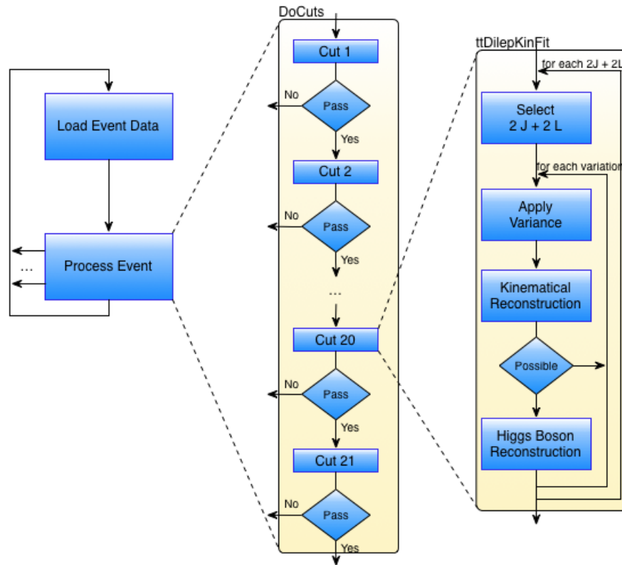
Figure 3.1: Schematic representation for the t\bar{t}H_{dilep} application flow.
