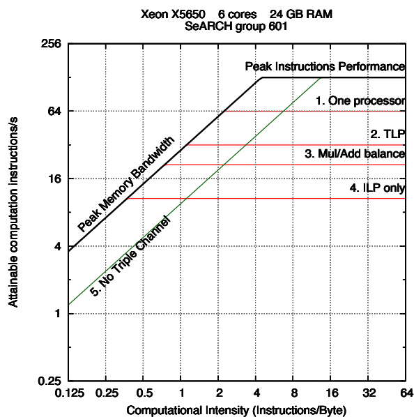
Figure C.1: Roofline models for the compute-601 system used in the ttDilepKinFit computational characterization.
