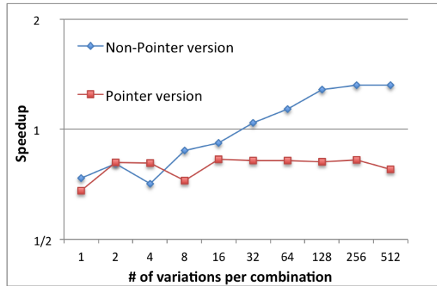
Figure 4.8: Speedup provided by using hardware multithreading for the non-pointer version.
