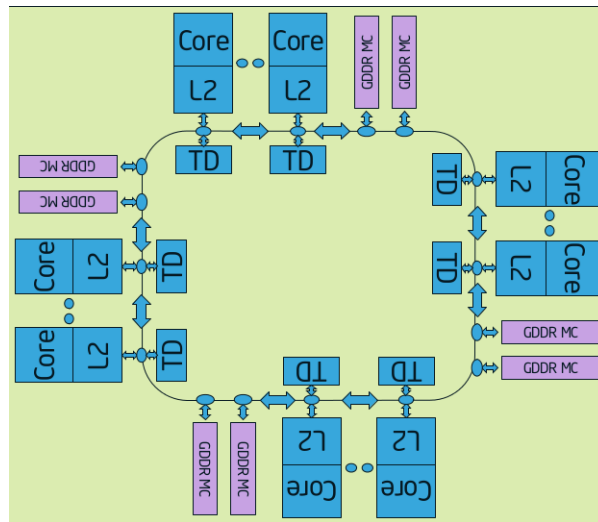
Figure 2.5: Schematic representation of the Intel MIC architecture.
