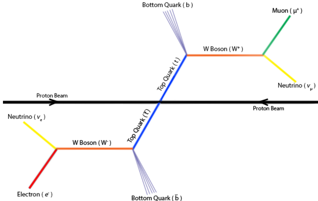
Figure 1.1: Schematic representation of the t\bar{t} system.
