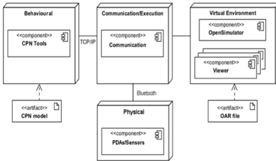
Figure 2.1: Logical architecture of the execution environments in APEX framework (from [Sil12])
