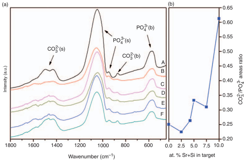
Figure 3. (a) FTIR spectra of the coatings: (A) Si0Sr0, (B) Si2.5Sr0, (C) Si2.5Sr1.75, (D) Si2.5Sr2.5, (E) Si2.5Sr5.0 and (F) Si2.5Sr7.5. and (b) \text{CO}_3^{2-}/\text{PO}_4^{3-} areas ratio obtained from the spectra.
