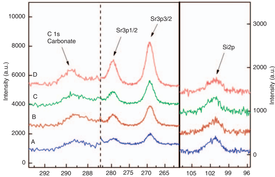
Figure 4. High resolution XPS spectra of the C 1s associated to carbonate groups (a), Sr 3p (b) and Si 2p (c) electronic transitions, for: (A) Si2.5Sr1.75, (B) Si2.5Sr2.5, (C) Si2.5Sr5.0, (D) RSi2.5Si7.5.
