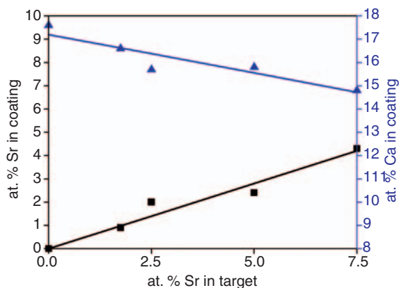
Figure 5. Sr (■) and Ca (▲) at. % in the coatings obtained by XPS as a function of the at. % Sr in the target.
