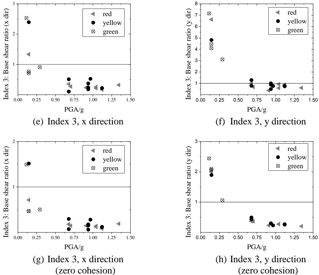
Figure 4. Indices for clay brick URM churches in the Canterbury earthquakes
