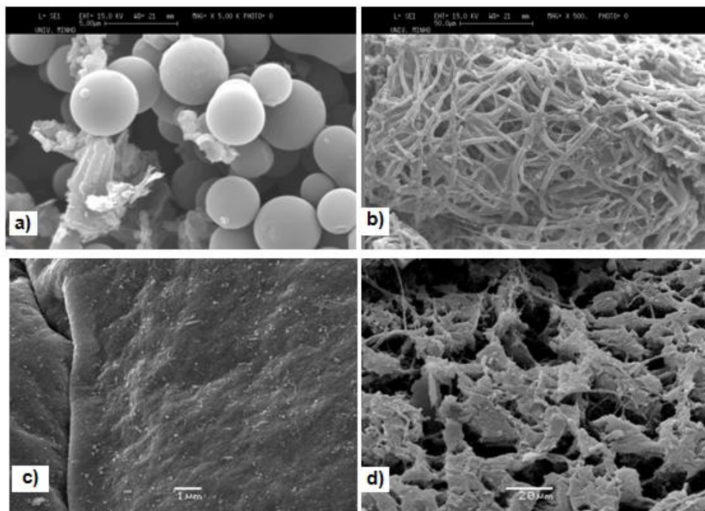
Fig. 4 Scanning electron microscopy of complex pellets of A. discolor , after 7 days of incubation. (a) Black core inside both pellets (5 \mu\text{m} ); (b) fungal mycelia on the surface of complex pellets (50 \mu\text{m} ); (c) surface of coated pellets (1 \mu\text{m} ); (d) fungal mycelia under the surface of coated pellets (20 \mu\text{m} ).
