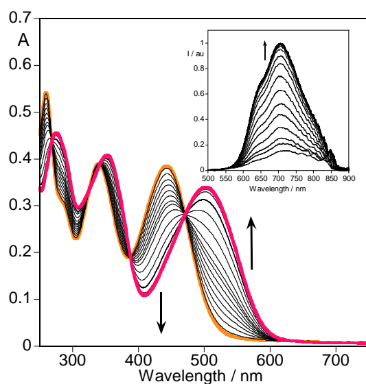
Figure 1. Changes in UV-vis and fluorescence (inset) spectra for compound 2a ( 1.75 \times 10^{-5} M) in CH 3 CN with addition of CH 3 CN solution of [(Bu) 4 N]F. Absorptions read at 444 nm and 503 nm.
