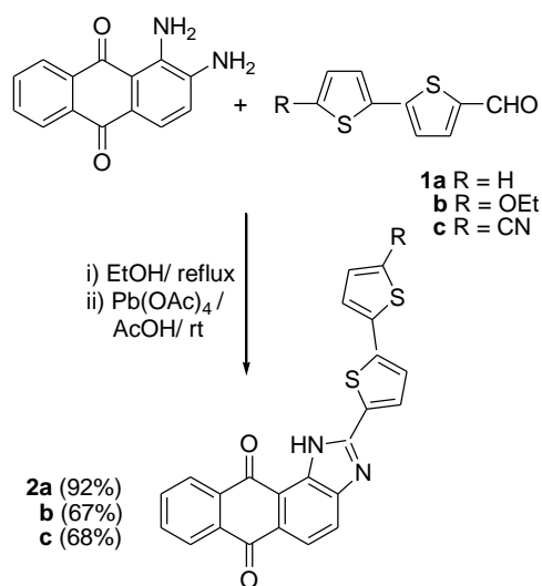
Scheme 1. Synthesis of sensors 2
