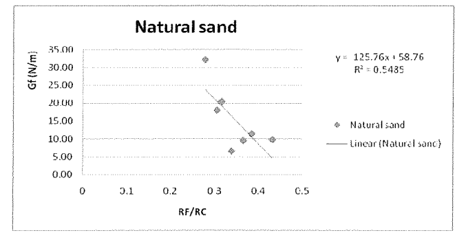
Figure 10. Natural sand. Ratio between RF/RC and the fracture energy.
