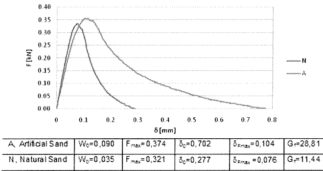
Figure 5. Cement mortars. Resistance class M5: M5_C_A; M5_C_N. Average values of fracture energy.
