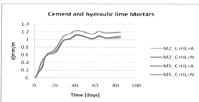
Figure 4. The shrinkage evolution of the cement and hydraulic lime mortars.
