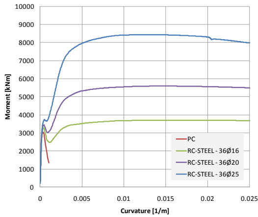
Figure 9. Moment vs. curvature for PC and RC-STEEL cases.
