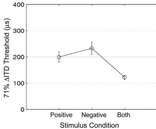
Fig. 4. Results from experiment 1 averaged across three observers. The abscissa represents the stimulus condition, with the ITD carried by: 1) the positive envelope slopes, 2) negative slopes, and 3) both slopes (standard SAM waveform). The ordinate represents interaural delay threshold. Error bars show \pm 1 standard deviation.
