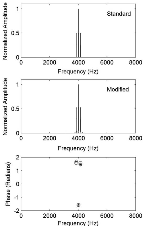
Fig. 3. Amplitude and phase spectra of a standard SAM tone (top panel) and modified (middle panel) waveform with the latter's envelope extended by 250 \mu s in the negative modulation slope. The phase spectra (bottom panel) at the carrier and sideband frequencies are shown by circles (standard SAM) and asterisks (modified waveform).
