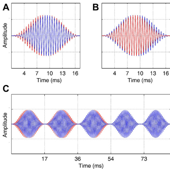
Fig. 6. Panels A and B represent the types of modulation cycles used in experiments 2 and 3 in which interaural delays were selected on each trial from a normal distribution separately for the positive and negative slopes. Panel A shows a sample modulation cycle with ITDs of +450 and -200 \mu\text{s} in the positive and negative slopes respectively, and panel B shows ITDs of -210 and +435 \mu\text{s} . The delays shown in this figure are larger than those used in the experiment to facilitate visual inspection. Panel C shows the first five cycles of a representative waveform used in experiment 3, with the first 3 cycles dichotic and the next two diotic (zero ITD).
