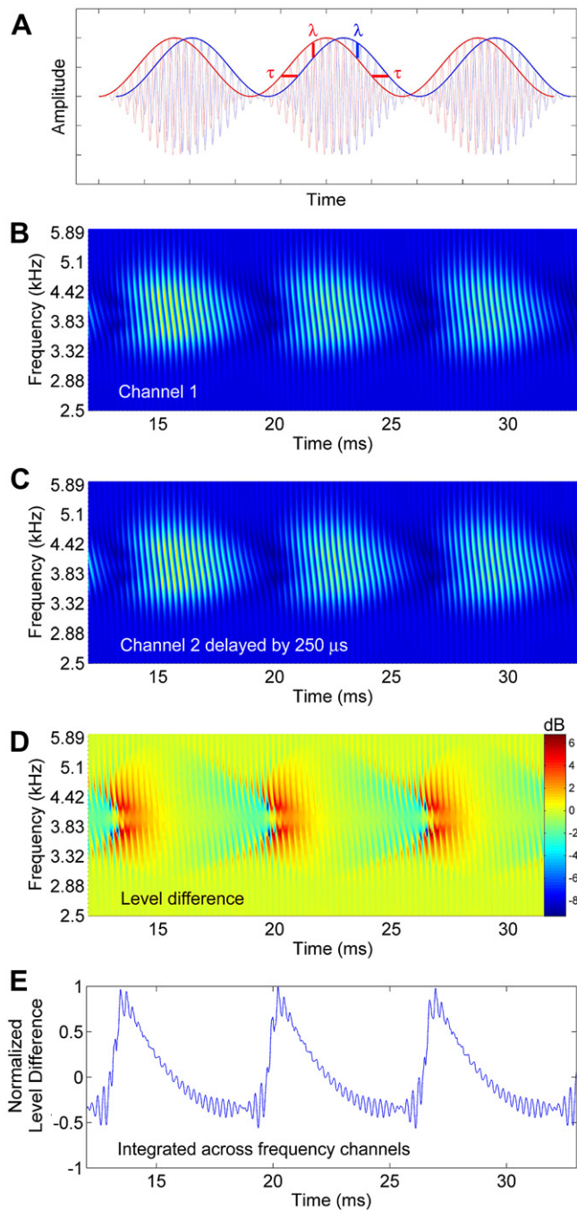
Fig. 1. Panel A shows a schematic of a dichotic sinusoidally amplitude-modulated (SAM) waveform with one channel (blue) delayed by \tau relative to the other (red). Note the presence of a concomitant interaural level difference cue \lambda favoring the blue waveform in the negative slope of the modulation envelope. Panel B shows the output of a computational model of the auditory periphery consisting of a GammaTone filterbank with 50 filters whose resonant frequencies were logarithmically spaced from 2.5 to 6 kHz, followed by an inner hair-cell model. The stimulus was a SAM waveform with a 4-kHz carrier modulated at 150 Hz. Activity is shown during the sustained part of the waveform after the 10-ms rise time. The striations result from ringing of the filters. Panel C shows the same waveform delayed by 250 \mu s. Panel D shows the predicted interaural level difference in dB (from panels B and C). Panel E shows level differences integrated across frequency channels (from D) and normalized to a maximum value of 1. (For interpretation of the references to colour in this figure legend, the reader is referred to the web version of this article).
