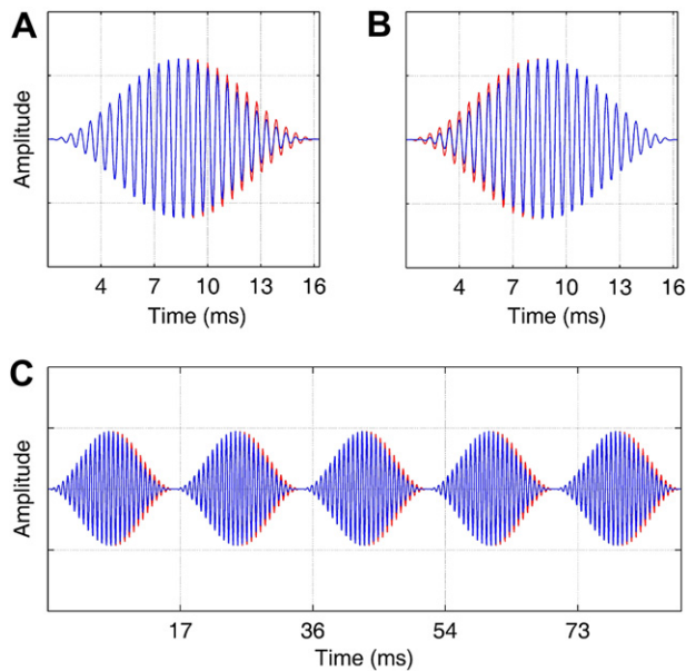
Fig. 2. Stimuli used in experiment 1 contained an interaural delay either in the negative (A) or positive (B) modulation slope, and were generated from concatenation of individual modulation cycles whose envelope peaks were extended by the desired interaural delay (C). The blue waveforms are plotted on top of the red waveforms, with the blue representing the stimulus delivered to one ear, and the red the stimulus to the other ear. The stimulus shown in panel C is a 4-kHz carrier modulated at 150 Hz with a 250- \mu s interaural delay applied to the negative slope. (For interpretation of the references to colour in this figure legend, the reader is referred to the web version of this article).
