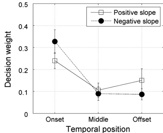
Fig. 7. Results from experiment 3 averaged across three observers. Decision weights are shown for ITDs in the first 3 modulation cycles (onset), the 3 modulation cycles in the center of the waveform, and the final 3 modulation cycles (offset). The parameter is modulation slope (positive or negative). The stimulus had a modulation rate of 100 Hz and a duration of 300 ms, resulting in 30 full cycles, 21 of which were diotic. Error bars show \pm 1 standard deviation. Note that the sum of the weights across conditions is equal to one.
