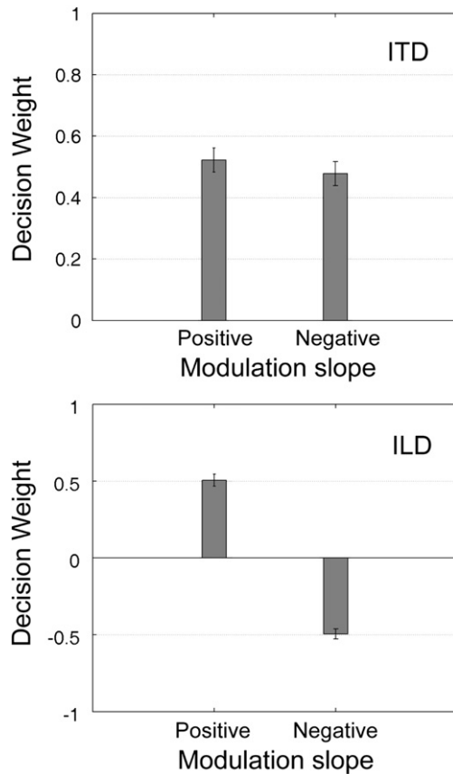
Fig. 5. Results from experiment 2 averaged across three observers. Top panel plots estimated decision weights associated with ITDs in the positive and negative modulation slopes ( \tau in Panel A of Fig. 1). Bottom panel shows decision weights associated with ILDs in the positive and negative modulation slopes ( \lambda in Fig. 1). Error bars show \pm 1 standard deviation.
