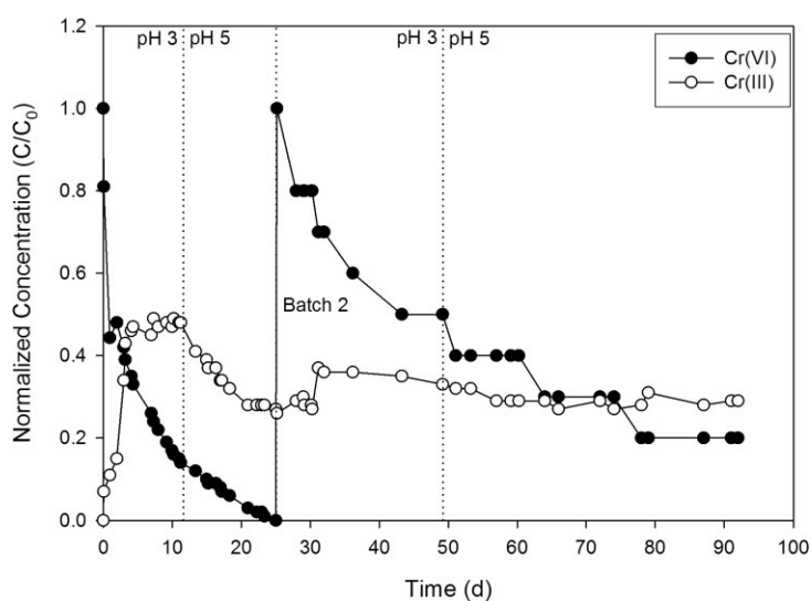
Figure 3. Cr concentration evolution during the laboratory-scale batch assay at pH 3 and 5 with biomass concentrations of 5 \text{ g L}^{-1} in the two batches (E2).
